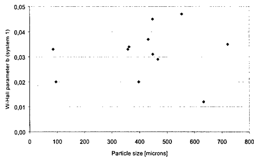
Fig. 49: W-Hall parameter b plotted versus particle size (system 1)
