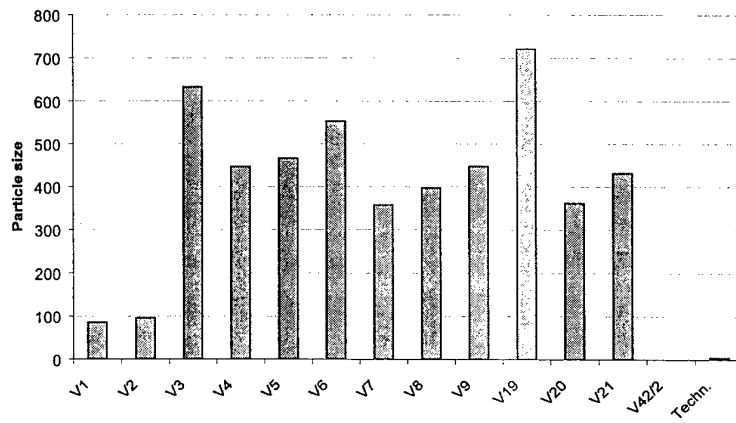
Fig. 21: Particle sizes of the HMX samples [ \mu\text{m} ]; The particle sizes of the samples V1 and V2 are comparable lower
