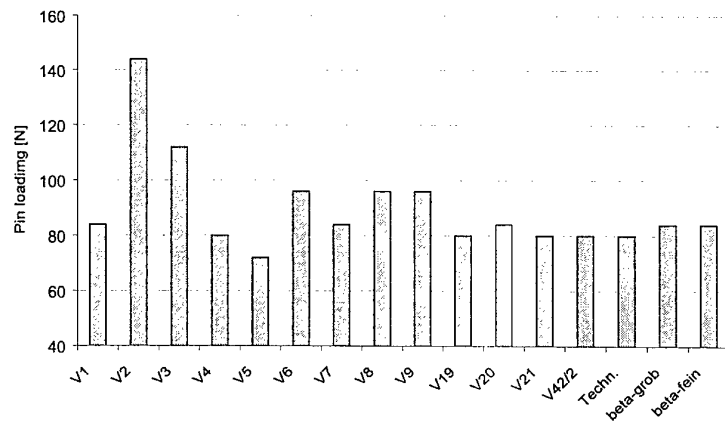
Fig. 23: Friction Sensitivity determined according to BAM
