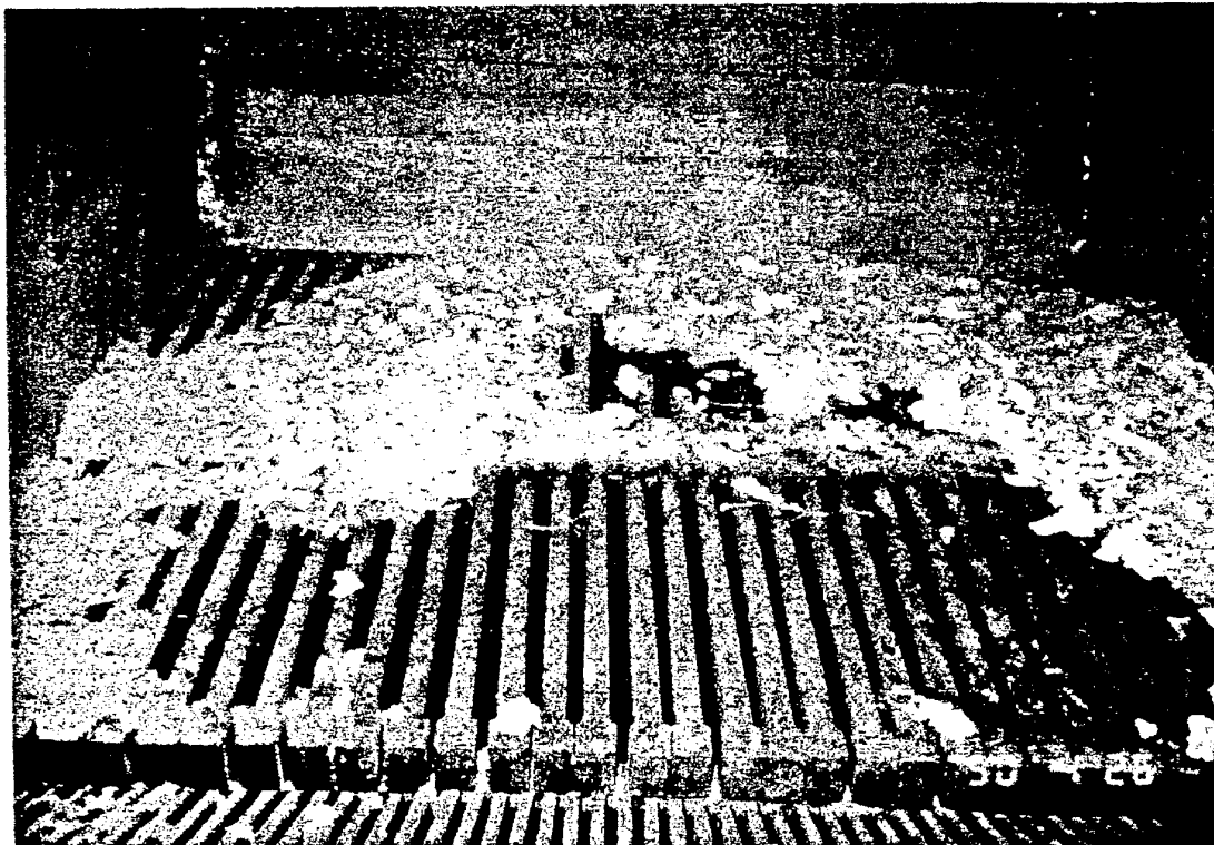
Fig. No. 6 Grate System for handling Burnable Waste only
