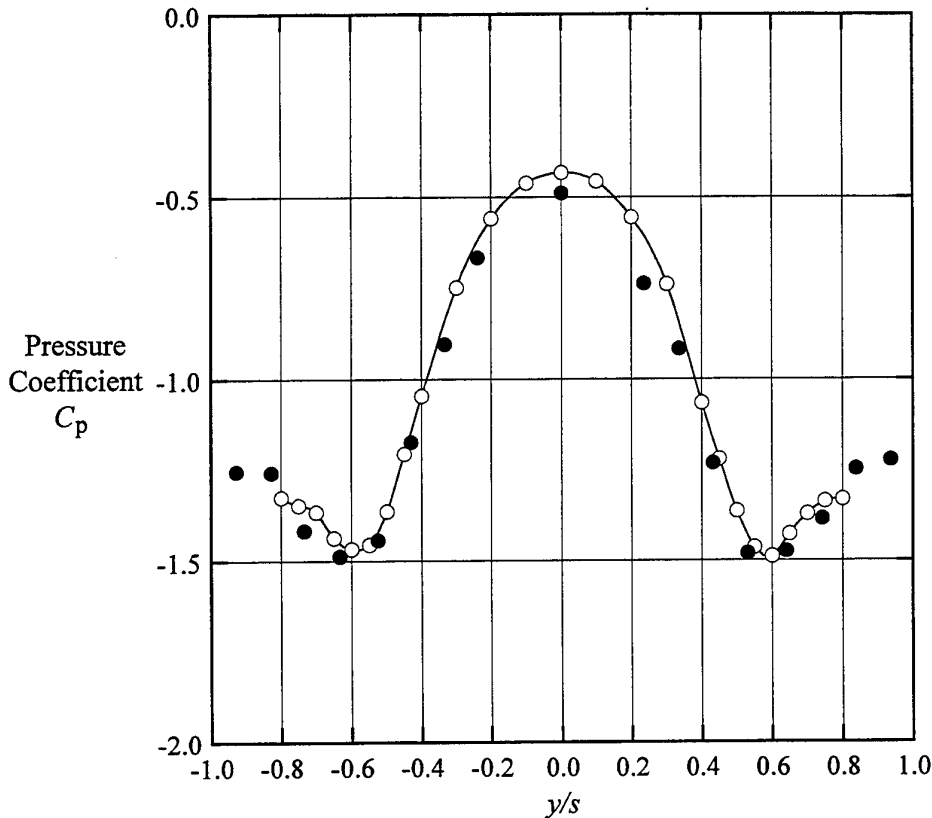
Figure 8. Comparison between pressure coefficients measured on a delta wing in the AMRL water tunnel and in a wind tunnel for \alpha = 30^\circ and x/c = 0.75 . ○ Water-tunnel data; ● wind-tunnel data (Atashbaz & Ahmed, 1997).
