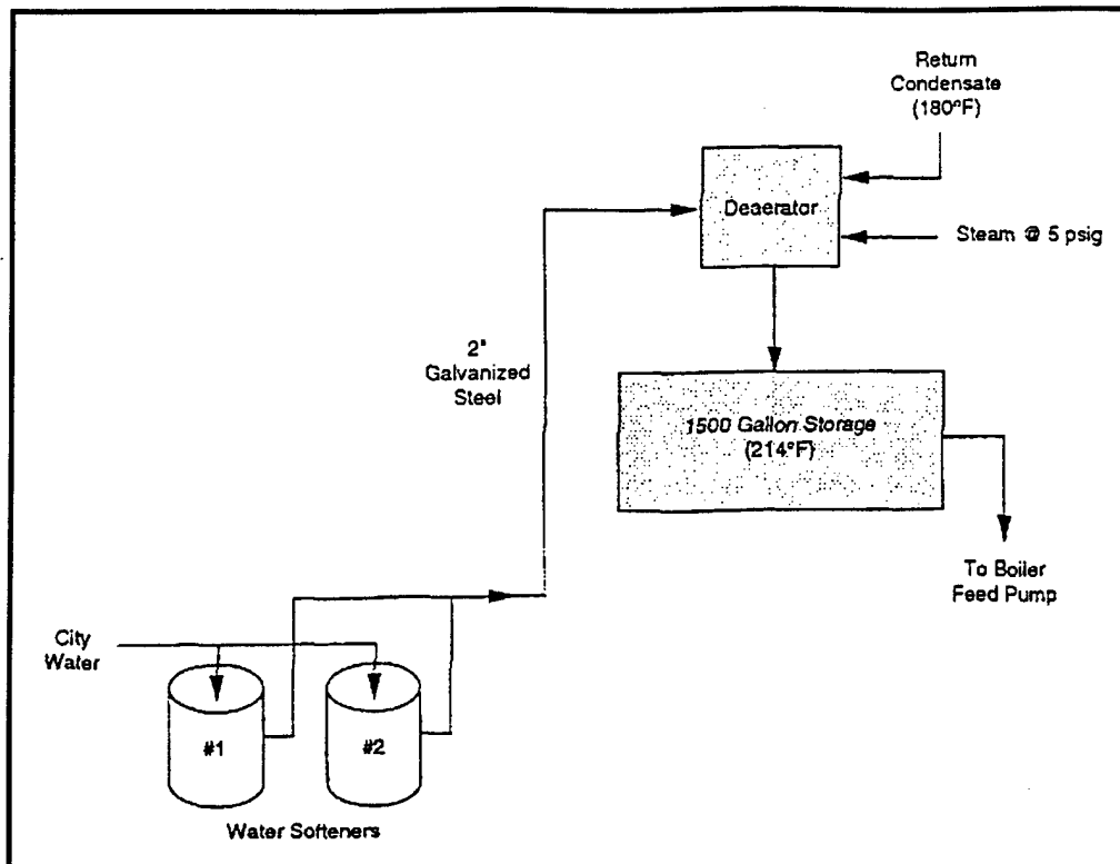
Figure 2. Boiler feed water process diagram.
