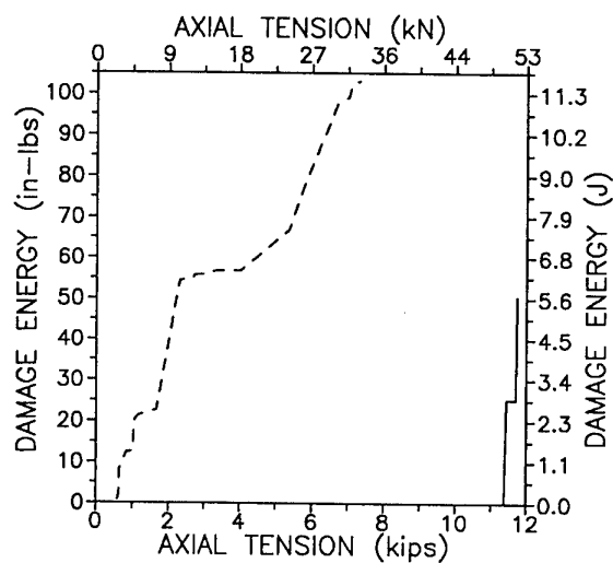
Figure 12 Exhausted Damage Energy under Tension Graphite-epoxy: AS-4/HMHS[0/90/±45] S Solid line: unstiffened shell Dashed line: integrally stiffened shell
