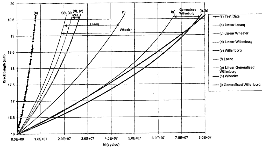
Figure 5 Load interactions predicted by the different models
