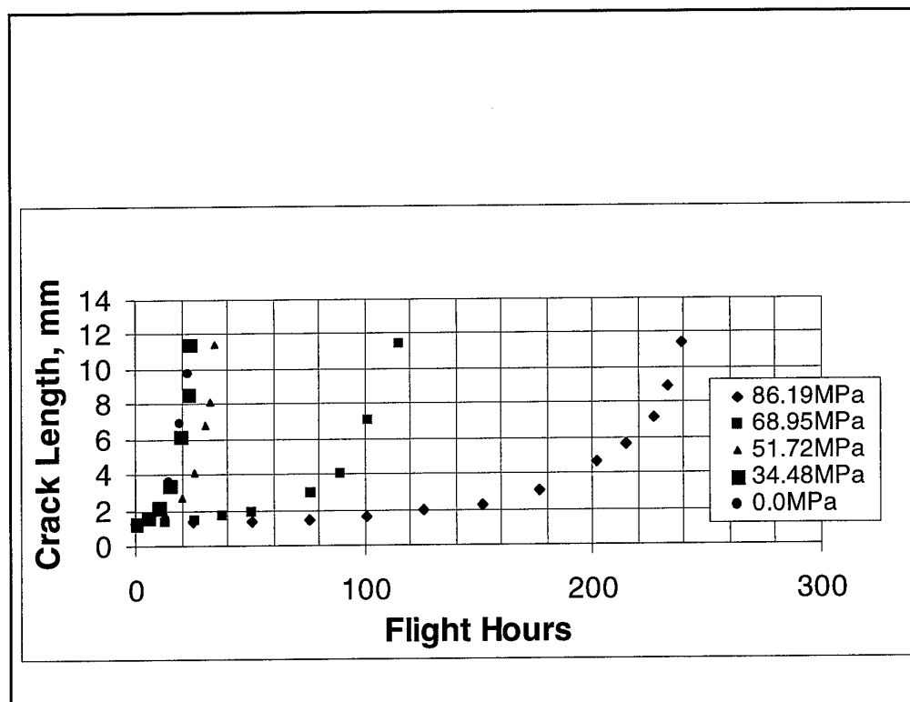
Figure 7 Effects Of Stress Range Truncation
