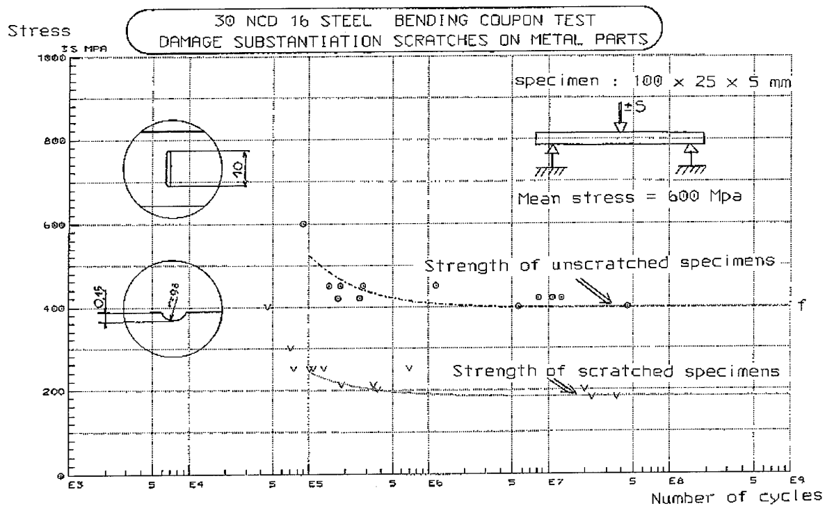
Figure 7 : Fatigue Curve on Flawed Specimens
