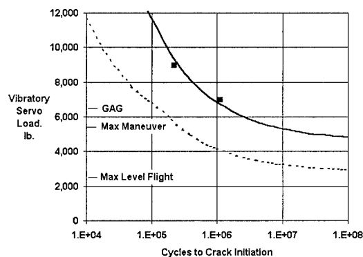
Figure 5. Crack Re-Initiation on Servo Beam Rail
