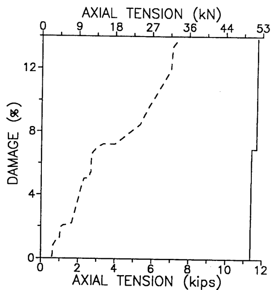
Figure 11 Damage Progression under Axial Tension Graphite-epoxy: AS-4/HMHS[0/90/±45] S Solid line: unstiffened shell Dashed line: integrally stiffened shell
