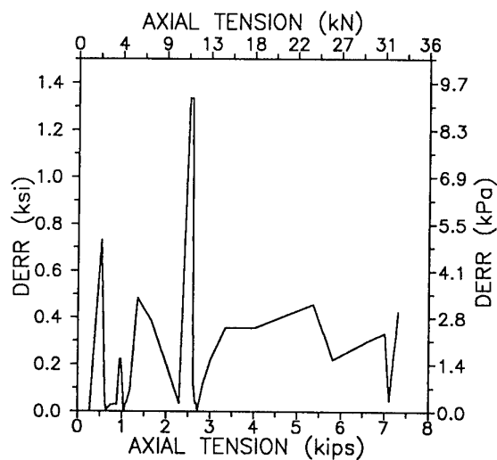
Figure 13 Damage Energy Release Rates under Tension Graphite-epoxy: AS-4/HMHS[0/90/±45] S Solid line: unstiffened shell Dashed line: integrally stiffened shell
