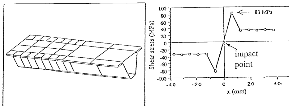
(a) Distribution of shear along the stiffener
