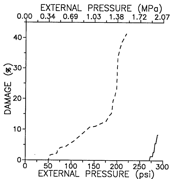
Figure 14 Damage Progression under External Pressure Graphite-epoxy: AS-4/HMHS[0/90/±45] S Solid line: unstiffened shell Dashed line: integrally stiffened shell
