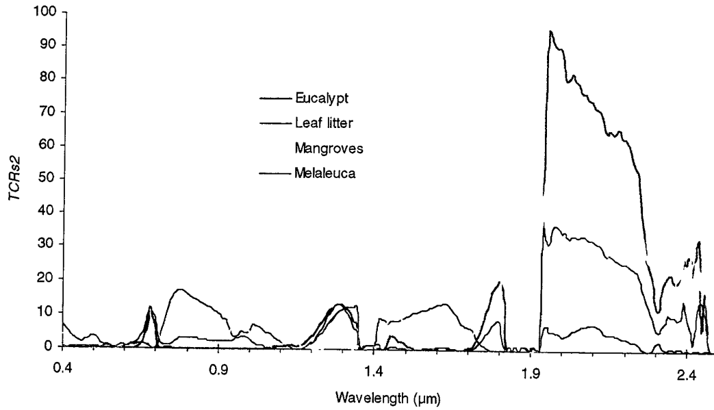
Figure C.3. TCRs 2 separation of green camouflage against background
