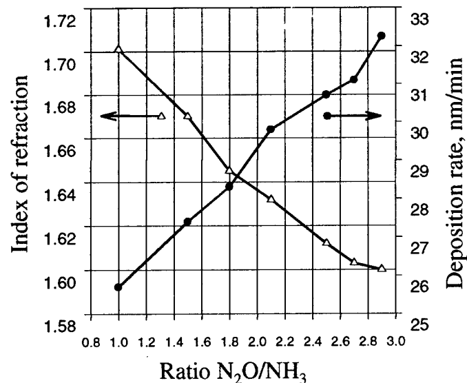
Fig. 4. Characteristics of silicon oxynitride films as a function of N_2O/NH_3 ratio.
