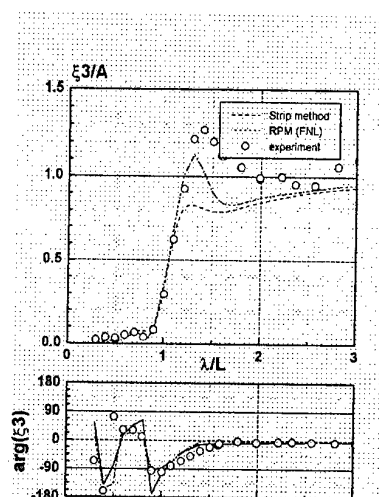
Fig.5 Heave motion at F_n = 0.2 , \chi = 180 degs.
