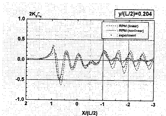
Fig.3 Steady wave distribution along longitudinal axis at F_n = 0.2
