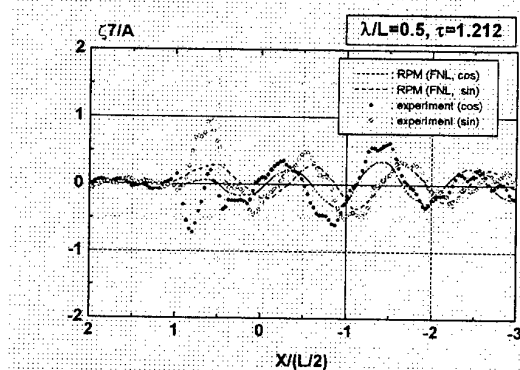
Fig.7 Diffraction wave at F_n = 0.2 , \chi = 180 degs.
