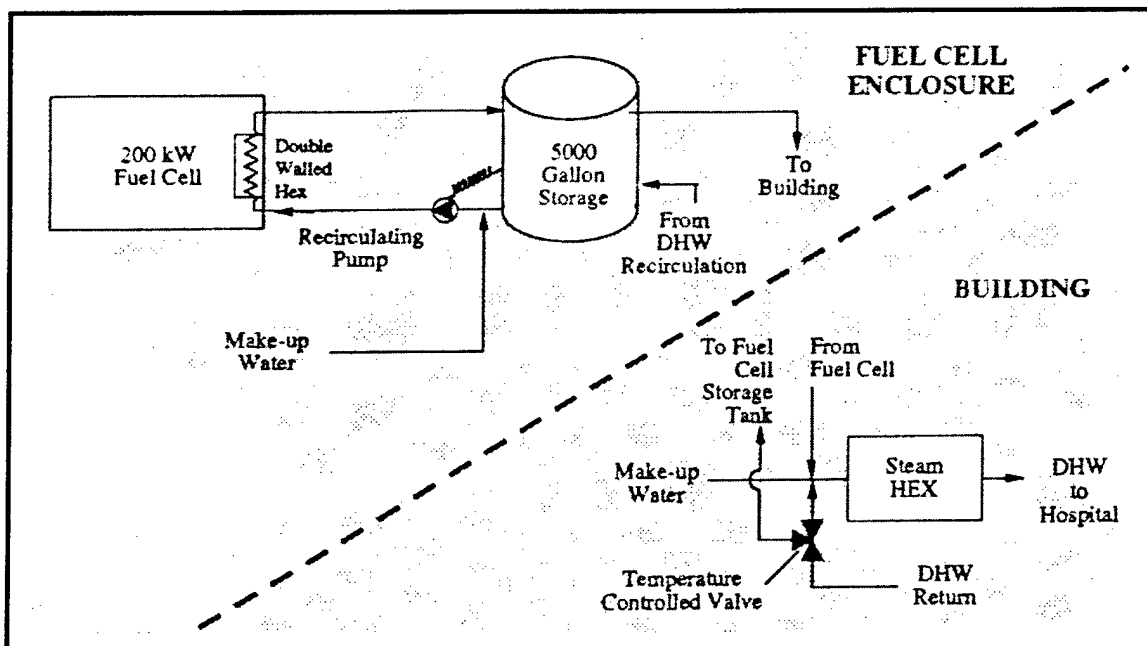
Figure 6. Fuel cell thermal interface—domestic hot water make-up and recirculation loop.
