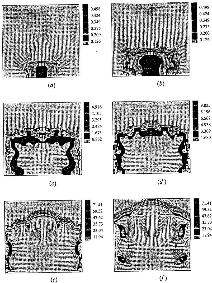
Figure 11 Calculated maps of the activation reaction intensity (in 10^{-2} \text{ 1/s} ) for successive stages of flame propagation in a cylindrical volume with a vertical axis of symmetry: (a) t = 9.7 \text{ ms} , (b) t = 14.2 \text{ ms} , (c) t = 16.25 \text{ ms} , (d) t = 16.35 \text{ ms} , (e) t = 16.46 \text{ ms} , (f) t = 16.54 \text{ ms}
