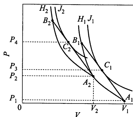
Figure 1 Hugoniots for different initial states of combustible gas. A_1(P_1, V_1) — initial state, A_2(P_2, V_2) — precompressed state, H_1 — initial shock Hugoniot, J_1 — initial detonation Hugoniot, H_2 — shock Hugoniot for precompressed state, J_2 — detonation Hugoniot for precompressed state, C_1 and C_2 — CJ points, A_1B_1 , A_2B_2 — Rayleigh lines
