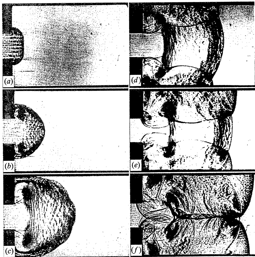
Figure 7 Schlieren photograph of detonation re-ignition due to Mach reflection behind an expanded cross-section. Expansion ratio 1:3. Unburnt gas mixture 2\text{H}_2 + \text{O}_2 + 70\% \text{ Argon}
