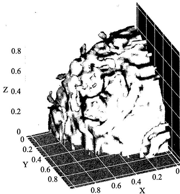
Figure 11 Three-dimensional calculations of instability of the interface between the detonation products of a spherical TNT charge and air
