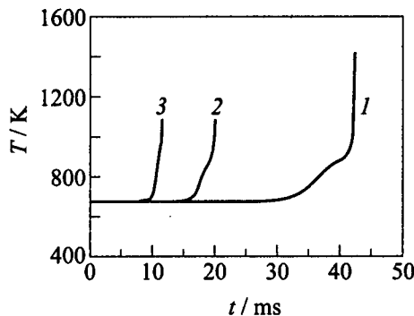
Figure 8 Predicted temperature histories of auto-ignition of fuel-lean mixture with \Phi = 0.5 (curve 1), stoichiometric (2), and fuel-rich mixture with \Phi = 2.0 (3) of ON = 90 at p_0 = 40 bar and T_0 = 670 K
