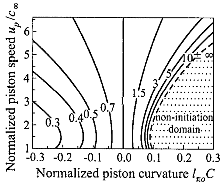
Figure 3 Level lines of the normalized induction time under impact by a curved non-accelerated piston (cf. Eq. (10b)). The dashed line represents the critical piston curvature (cf. Eq. (10f)) that produces infinite induction times, and separates the domains of non-initiation and initiation (negative and positive induction times, respectively). \gamma = 1.4 , T_a/T_\infty = 80 , Q_{pv}/r_\infty T_\infty = 30
