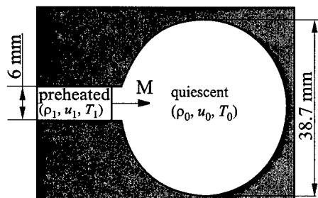
Figure 2 Schematic of a shock wave propagating into a combustible gas mixture
