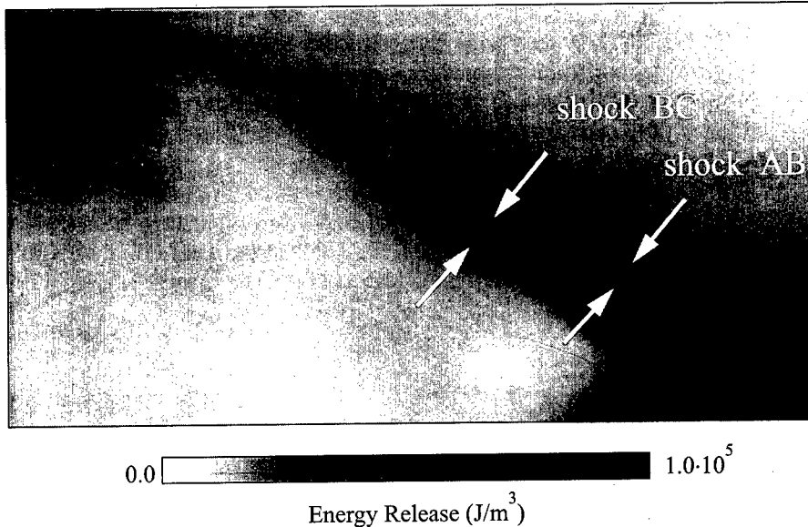
Figure 5 Enlargement of the energy-release contours in the region before triple-point collisions, resulting from complex multiple shock structure [18]
