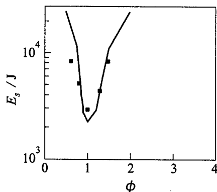
Figure 9 Measured (symbols) and predicted (curve) critical energies of direct initiation of spherical detonation in a hydrogen-air mixture at various equivalence ratios \phi
