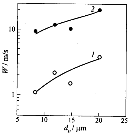
Figure 7 The correlation between the convective burning velocity and pore diameter for propellant A at 1 — P_x = 6 MPa and 2 — 16 MPa
