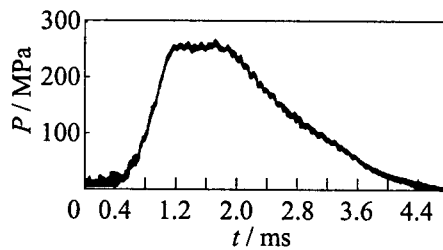
Figure 10 The pressure–time diagram with a plateau in 23 mm barrel system
