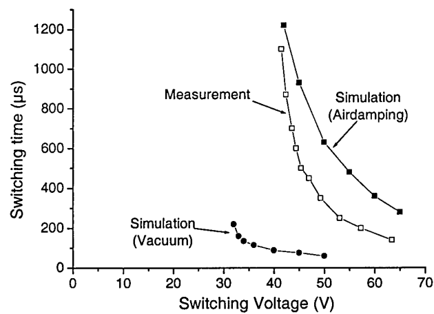
Figure 3: Measured switching time of diamond microswitch compared to simulation results excluding and including air damping effects.
