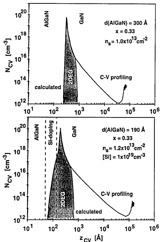
Fig.2: Calculated and measured carrier distribution of 2DEGs in pseudo-morphic, undoped and doped Al_{0.33}Ga_{0.67}N/GaN heterostructures with different barrier thickness.
