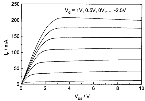
Fig. 2 Output characteristics
