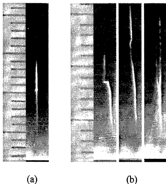
Figure 1 Typical Burning Trajectories of 1- \mu\text{m} Amorphous Boron Particles in; (a) CH 4 /O 2 /N 2 Flames and (b) CH 4 /NF 3 /O 2 /N 2 Flames ( T_{\text{amb}} = 2,020 \text{ K} , Each Graduation on the Scale is 1 mm)
