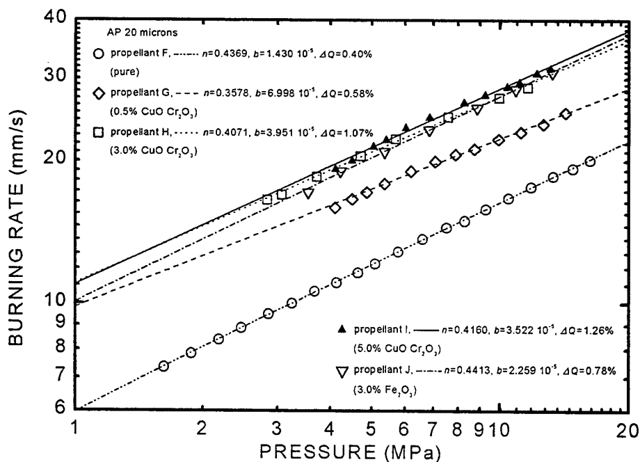
Fig. 1 Influence of Copper Chromate and Iron Oxide on medium-energy propellants (AP 20 \mu )
