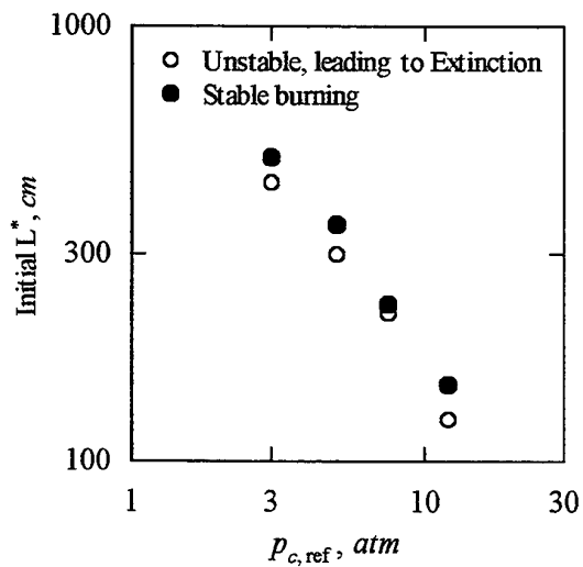
Figure 2. Stability diagram, showing regions of stable and unstable operation.
