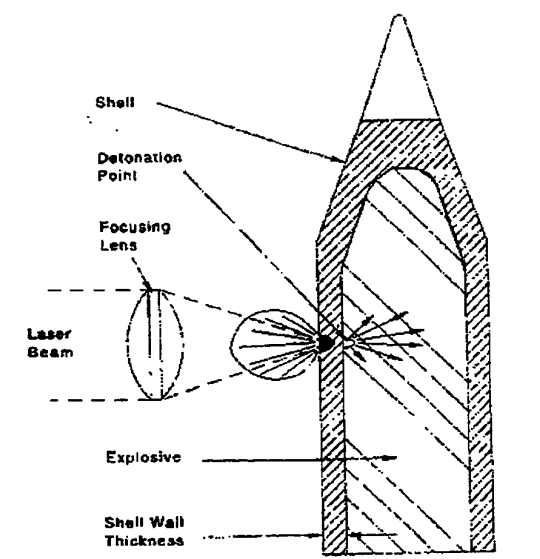
Fig. 2. Overall view of laser drilling into shell
