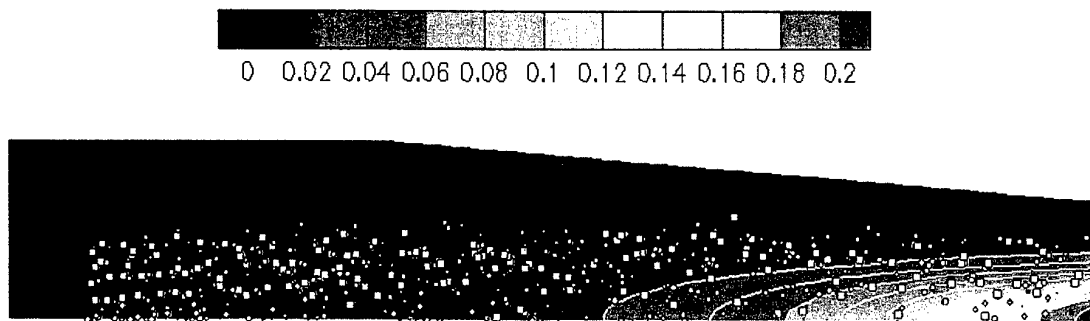
Two-phase flow computation in a simplified LPP – burned gas mass fraction and fuel drop locations
