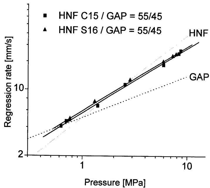
Figure 2: Regression rate of HNF/GAP propellants compared to that of neat HNF and GAP. ( \boxtimes , C15 coarse HNF; \blacktriangledown , S16 fine HNF)
