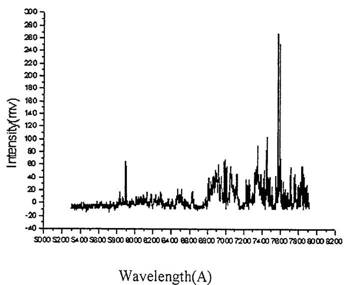
Figure 6: Spectrum for double-based propellants
