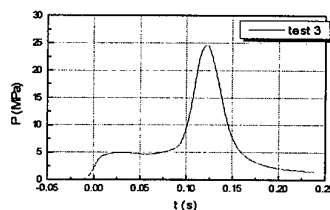
Fig. 7: Pressure-time trace of gas propagation process
