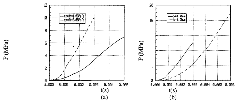
Fig.3 Pressure variation with the time in the crack tip (calculated)
