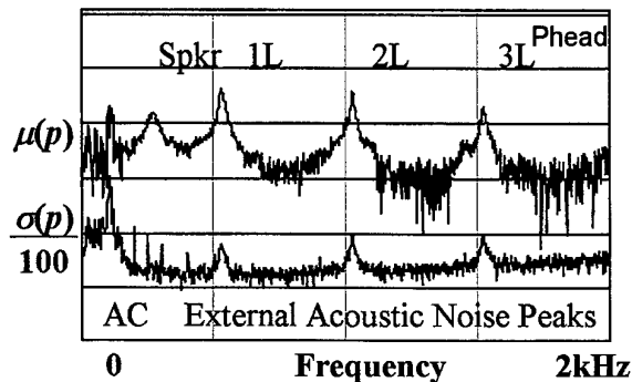
Fig. 1 Log Pressure Magnitude Mean and Standard Deviation.
