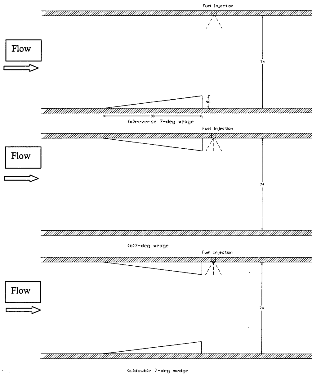
Fig.3 Test-chamber experiment configurations
