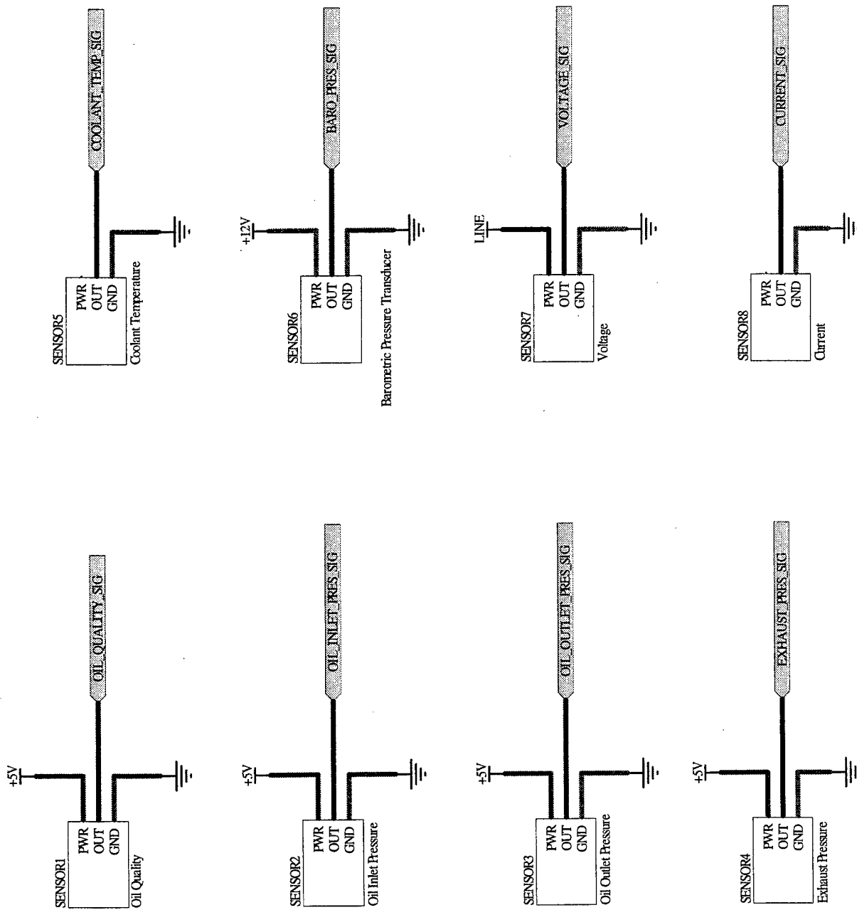
Figure E-4: 5V Module Signal Distribution
