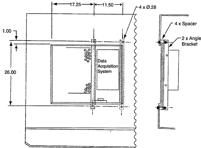
Figure D-5: DAS Mounting Diagram
