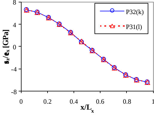
(a) Normal stress ( s_z ) with a_2 = 100
