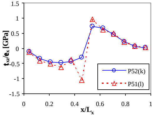
(c) Shear stress ( t_{xz} ) with a_2 = 100
