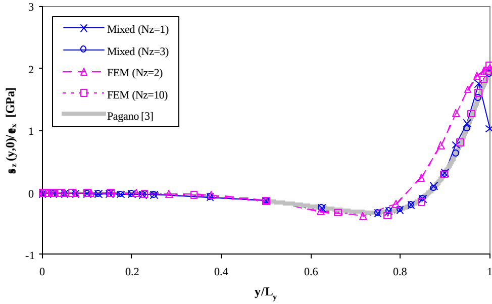
(d) Distribution of s_z along central plane ( z = 0 )
