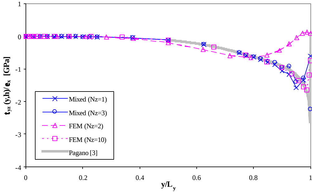
(c) Distribution of t_{yz} along [0/90] interface ( z = h )
