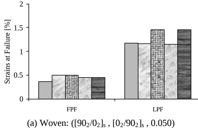
Figure 11. Numerical Prediction of Strains at FPF and LPF. Total strain is a sum of mechanical and residual strains.
