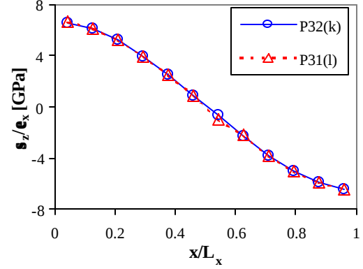
(b) Normal stress ( s_z ) with a_2 = 0
