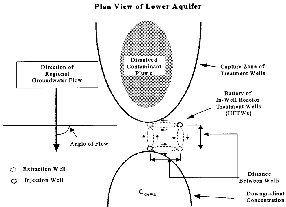
Figure 4.6. Two one-pair rows of treatment wells.
