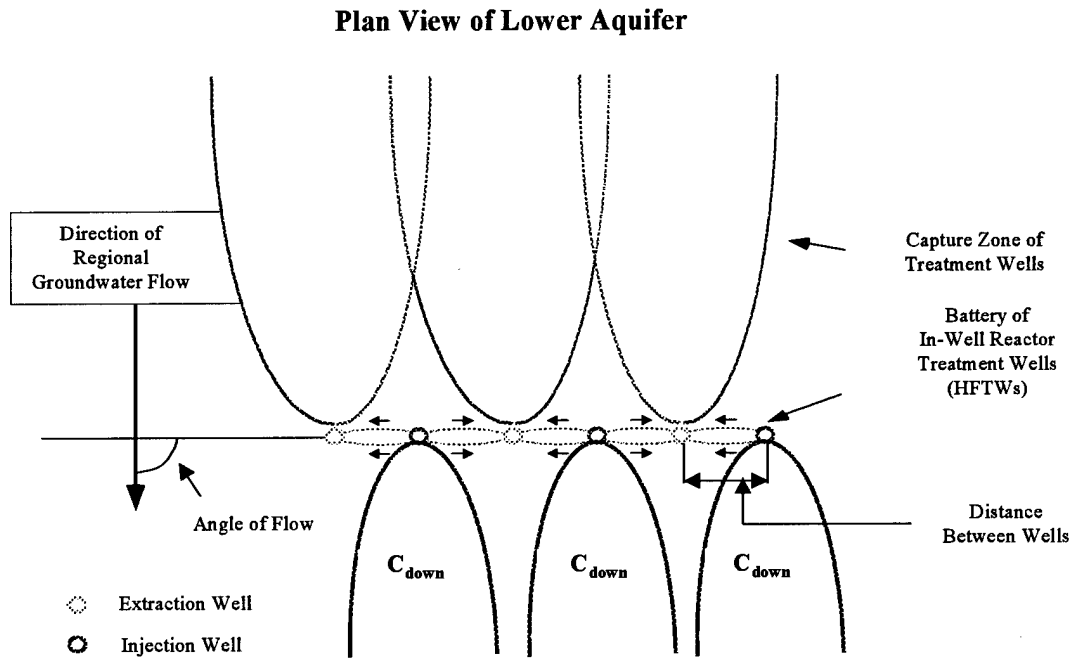
Figure 4.5 Row of multiple pairs of treatment wells
