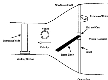
Figure 1a: Wind tunnel experimental setup
