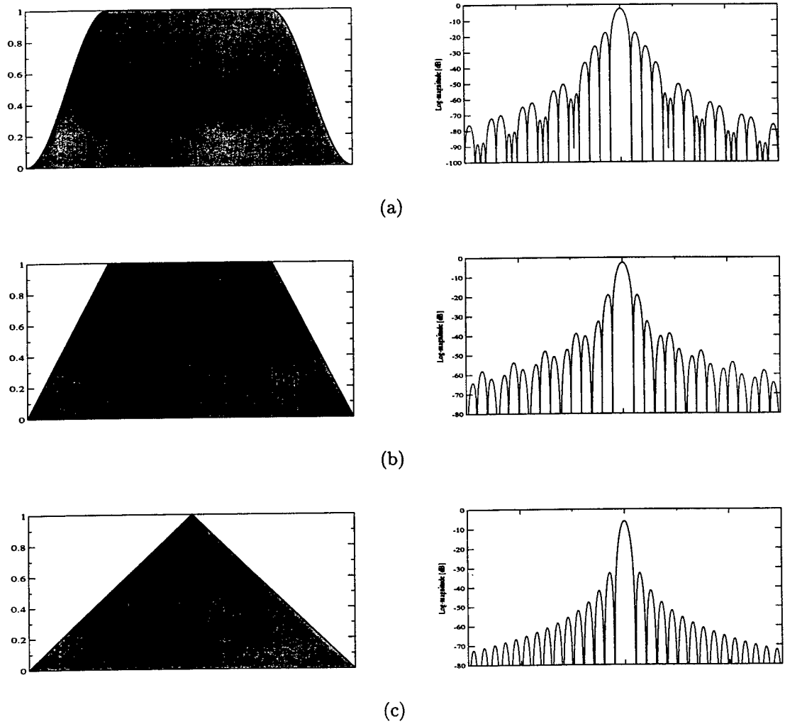
Figure 3.11: Apodizer transmittance and spectrum of (a) tukey, (b) trapezoid, (c) triangle.
