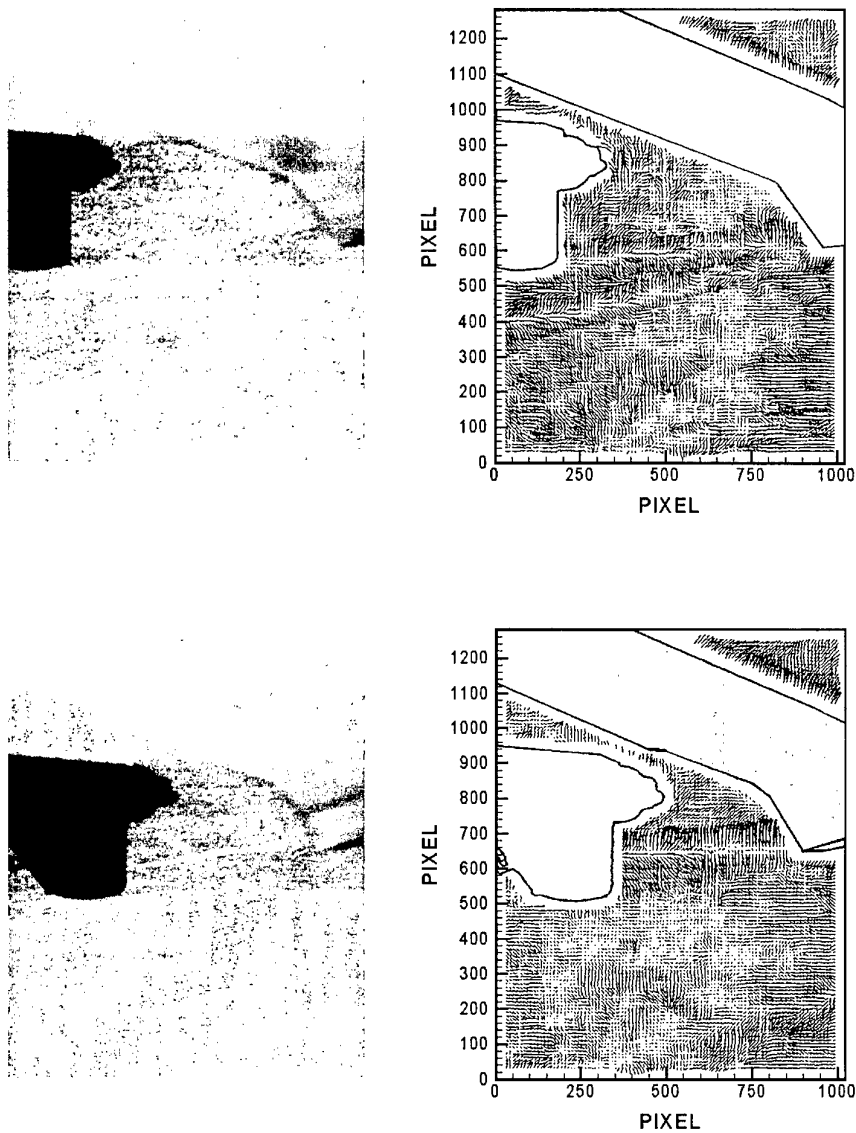
Fig. 38: Raw images from transonic blade tip over the background pattern (white dots on grey concrete) and the according density gradient plots
