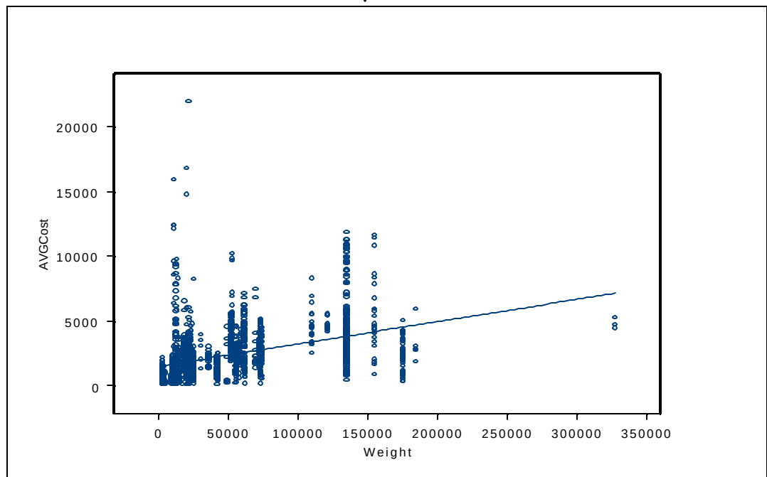
Figure 4.3 Scatter Plot for Average Annual Cost vs. Weight of Each TMS
