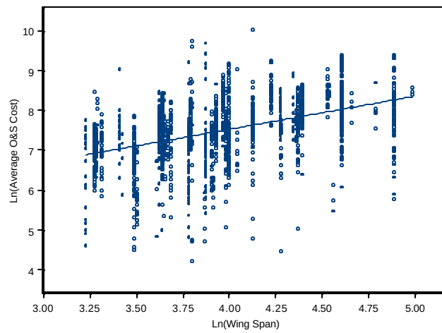
Figure 5.3 Scatter Plots with Regression Line for Two Independent Variables
