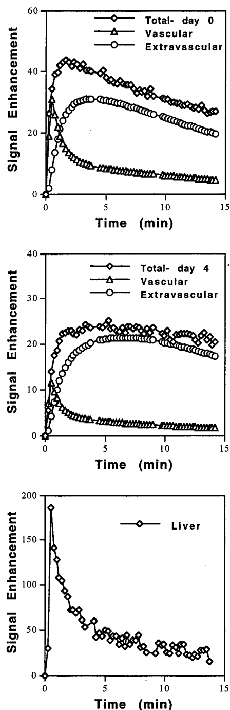
Fig. 3. The example of the pharmacokinetic analysis to separate the vascular vs. extravascular kinetics from the measured kinetics from the whole tumor. The kinetics from the control tumors, as shown in Fig. 2a, were analyzed. The total kinetics and the vascular and extravascular components at day 0 (a), day 4 (b), and the enhancement kinetics measured from the liver of the rat (c) are shown. By referencing to the liver kinetics (the distribution is in the entire extracellular space, assumed to be 24%), the vascular kinetics of the tumor was converted into vascular volume, which was about 4.2% at day 0 and 1.6% at day 4.
