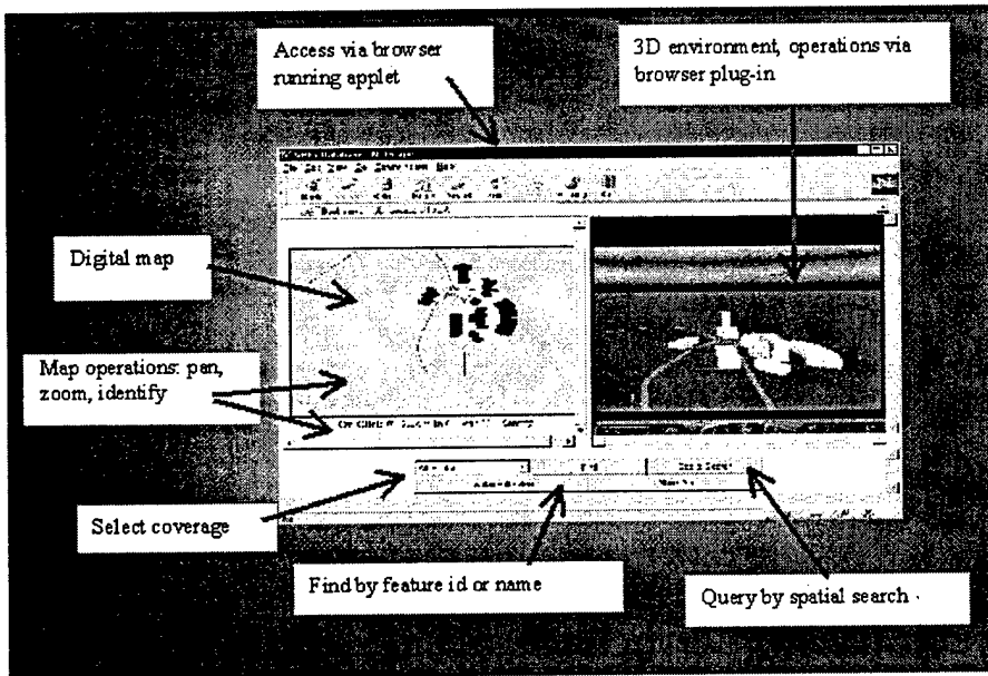
Figure 6. Prototype Mapping-3D Interface
