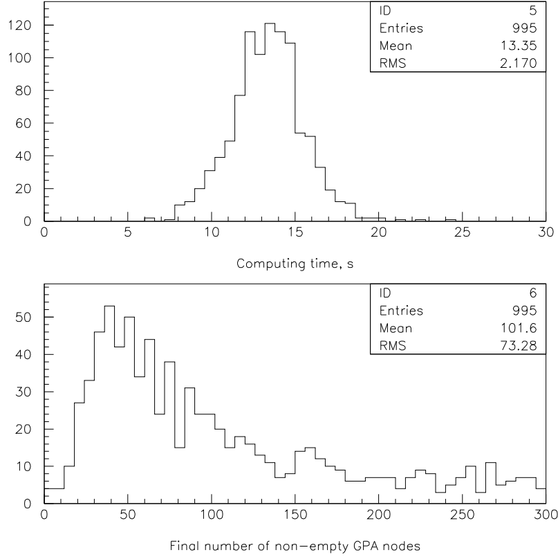
Figure 22: MC test results for c_y = c_z = 0.002 rad.
