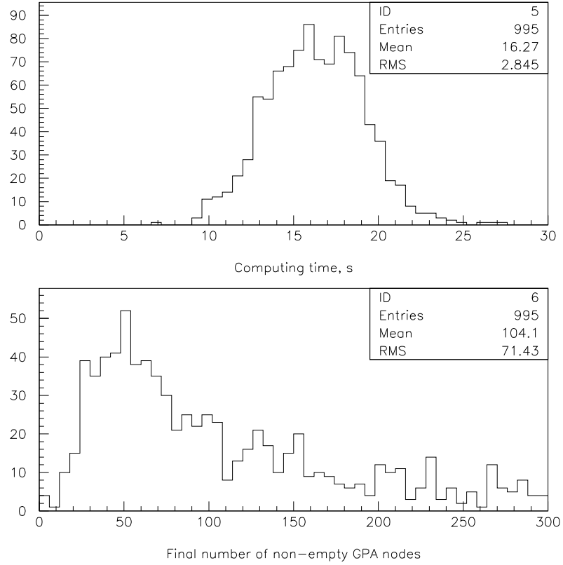
Figure 23: MC test results for c_y = c_z = 0.003 rad.
