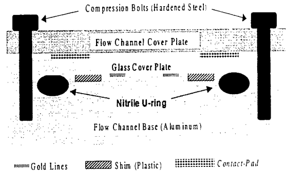
Fig. 6 Front view of the channel
