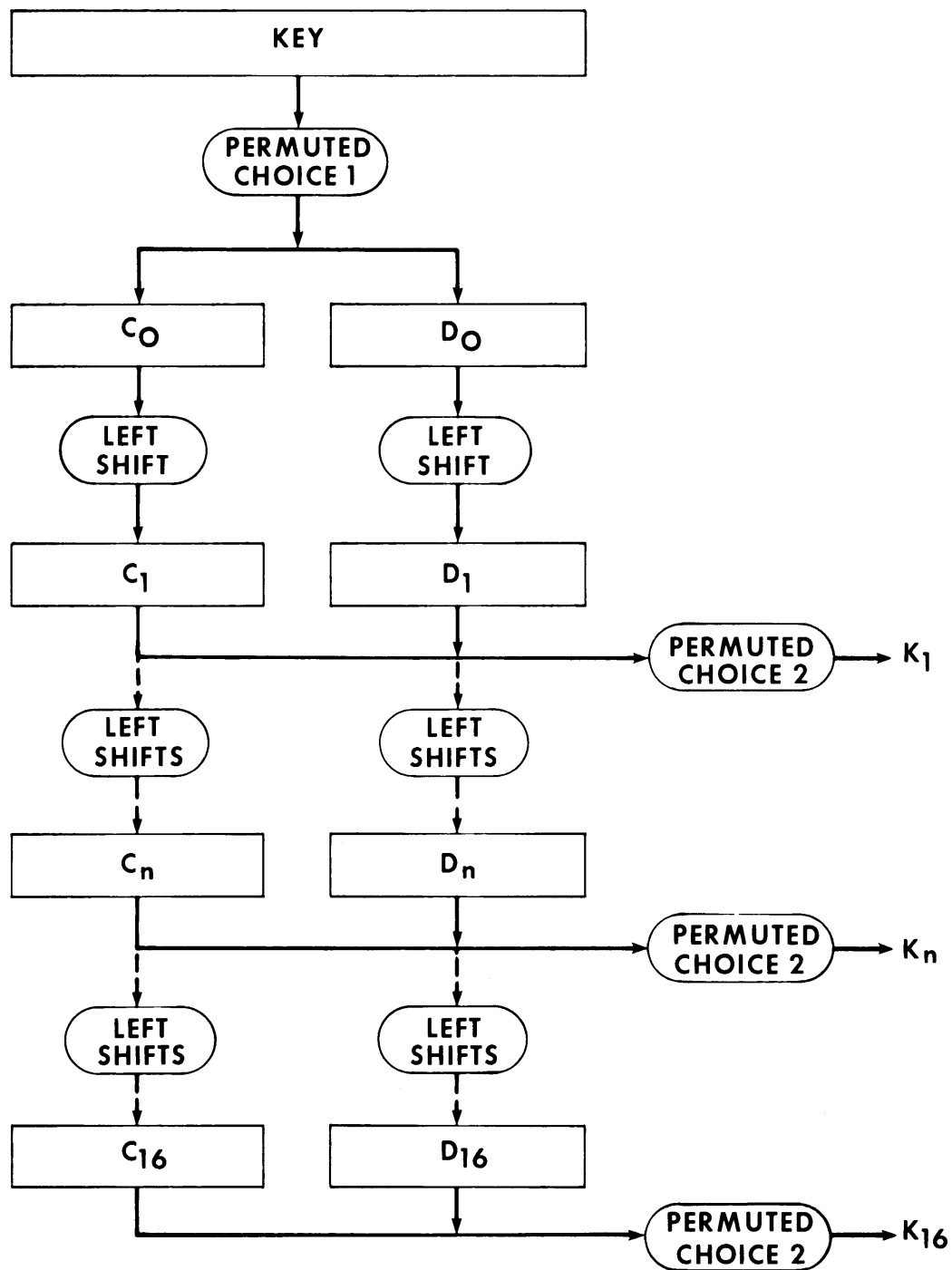
FIGURE 3. Key schedule calculation.
