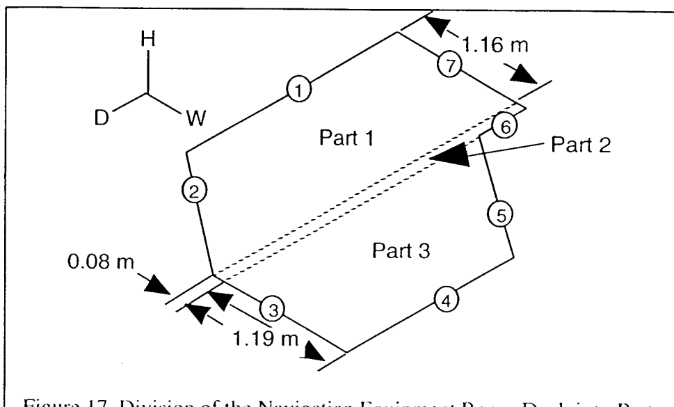
Figure 17. Division of the Navigation Equipment Room Deck into Parts
