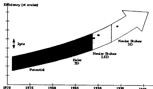
Figure 1: Impact of CFD on Snecma Commercial Fan Performance
