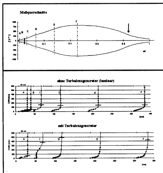
Fig. 7. Velocity profiles in the boundary layer at the wavy frontal part of the body measured by hot-wire anemometry. The horizontal lines indicate the boundary layer thickness corresponding to 99% of the velocity of the outer flow. Top: position of the measuring points; middle: velocity profiles without turbulence generator; bottom: with turbulence generator
