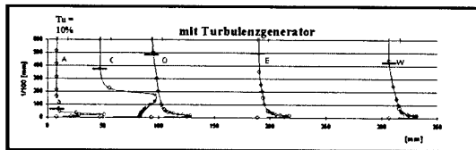
Fig. 8. Turbulence profiles. Transition was stimulated at ca. 5% of the body length. Points of measurement same as indicated in Fig. 7, with mean of the turbulent velocity fluctuation, free stream velocity, cf. [32]
