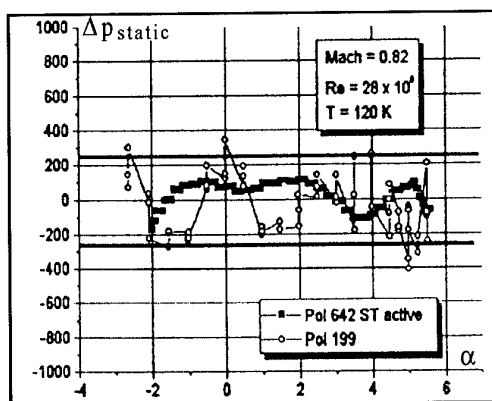
Figure 2: Stability of Static Pressure
