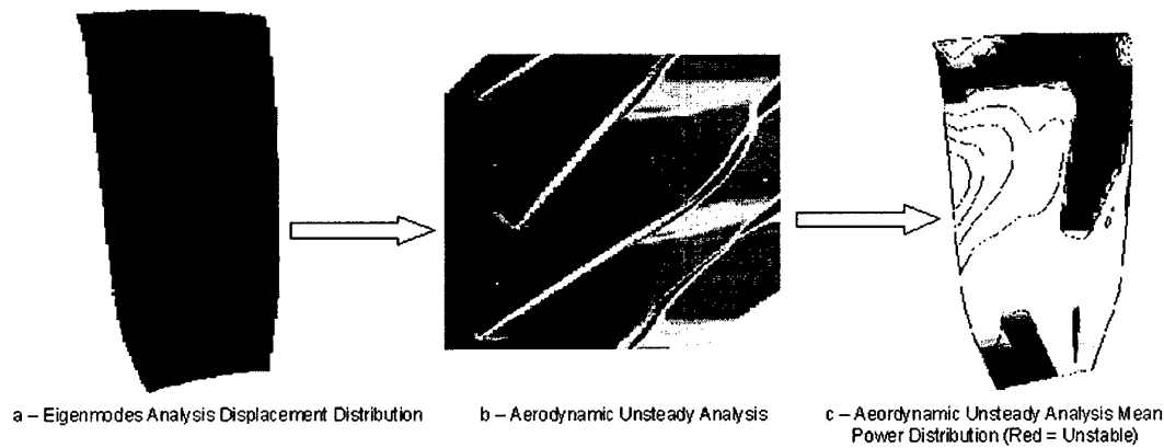
Figure 7: Aerodynamic Unsteady Analysis
