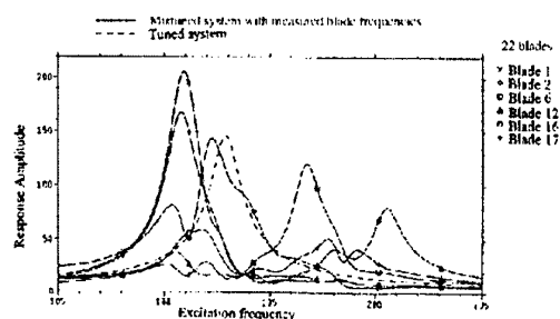
Figure 11: Mistuning influence on forced responses amplitude
