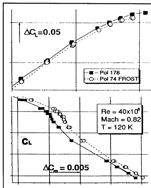
Figure 17: Influence of a Thin Layer of Frost on Aerodynamic Data
