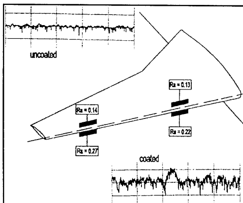
Figure 4: Wing Surface Roughness Measurements
