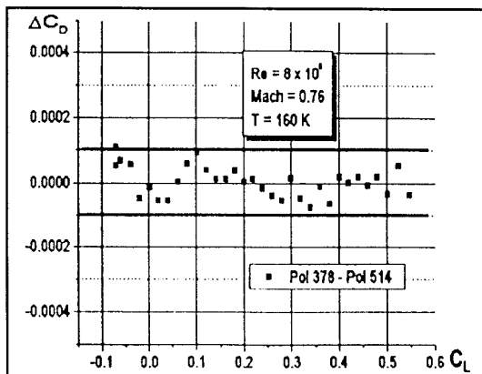
Figure 8: Deviation of Polars in Medium Term Repeatability Check
