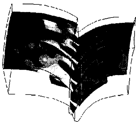
Figure 10: Computed flow field from unsteady 3D Euler code (IGV – Rotor 1 unsteady interaction at part speed)
