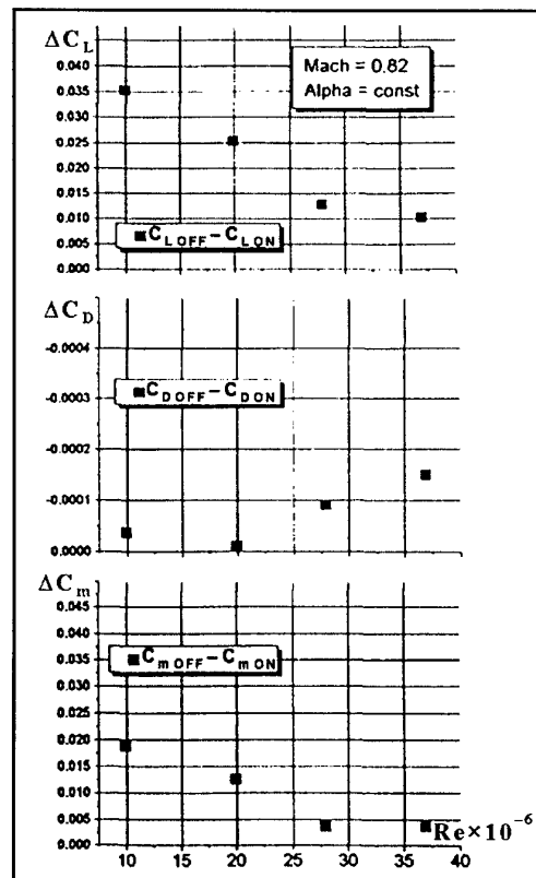
Figure 5: Influence of Coating on Aerodynamic Coefficients
