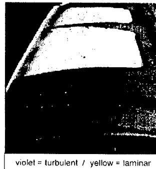
Infrared Image on Laminar Glove of Do228 with Transition
