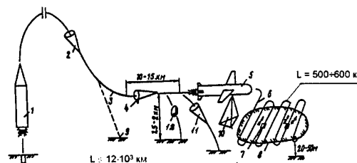
Fig. 1. The scheme of delivery of rescue means: 1 – rocket, 2 – nose cone, 3 – segment of transition, 4 – control flap, 5 – winged rescue-apparatus, 6 – search trajectory, 7 – objects of rescue, 8 – disaster area boundary, 9 – fictitious aiming point, 10 – directional diagram of navigation and supplementary reconnaissance means, 11 – heat-shielding body, 12 – bottom.
