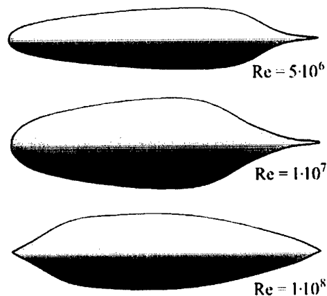
Fig. 14. Low drag bodies optimized for different Reynolds numbers by means of the Evolution Strategy (flow direction from left to right). (PhD, Th. Lutz)
