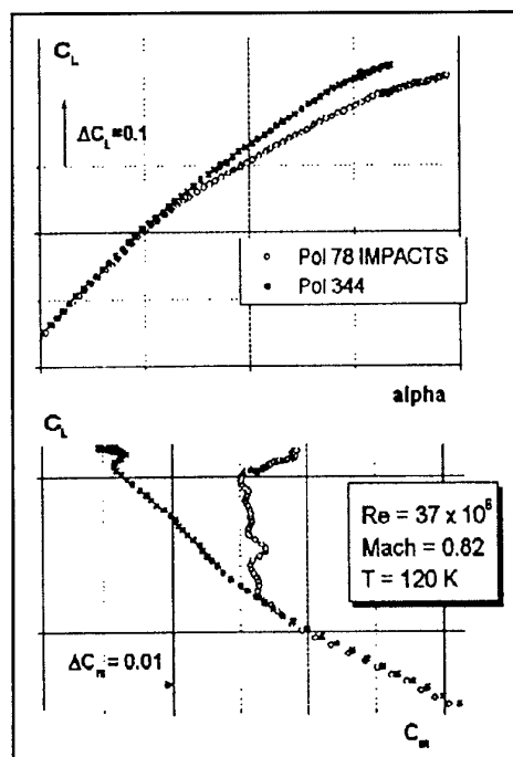
Figure 18: Influence of Model Surface Impacts on Aerodynamic Data
