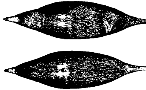
Fig. 5. Paint-flow visualisation on the body of rotation without (above) and with turbulence generator (below). Top view in both cases
