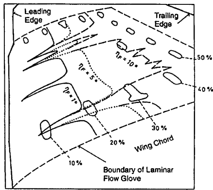
Changes of Transition Location by Increasing Flap Angles Observed in Flight by Infrared image Technique on ATTAS/VFW 614 Glove ( M = 0,34 , Re = 20 \times 10^6 )
