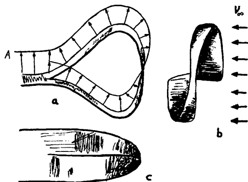
Fig. 27. Sketch of the bionic wing tip configuration "Split Wing Loop"; a – frontal view with lift distribution, b – side view, c – top view [59]
