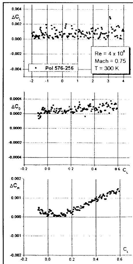
Figure 9: Long Term Repeatability
