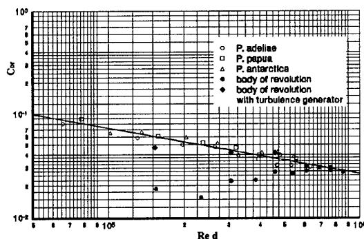
Fig. 2. Frontal drag coefficients plotted against Reynolds numbers. In this graph, Re was calculated by using the maximum diameter d as reference length
