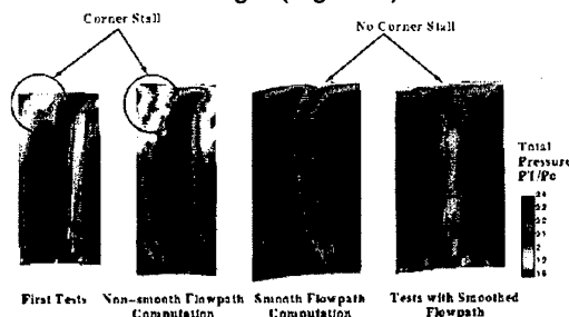
Figure 3: Compressor Variable Stagger Vanes - Experiment VS Computation Comparison
