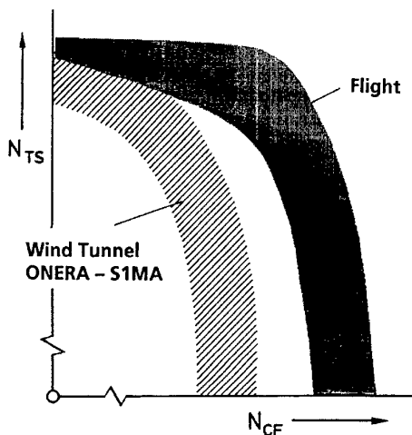
Limiting N-Factors for Transition Prediction in Flight and in S1MA Wind Tunnel for Swept Wings
