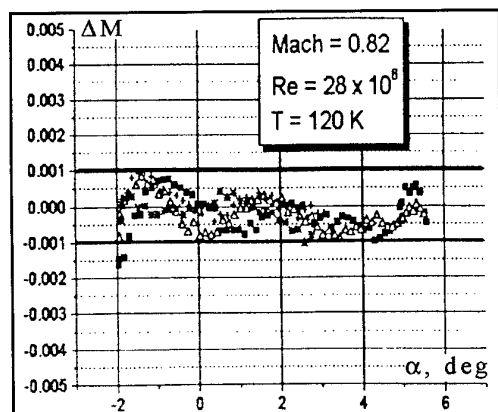
Figure 1: Mach Stability at High Reynolds Number
