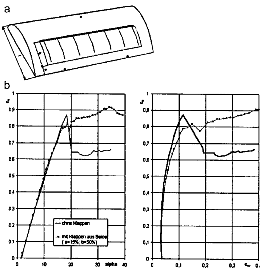
Fig. 19. Silk flap installed on a NACA 2412 airfoil (a), experimental data (b), solid line: without flap
