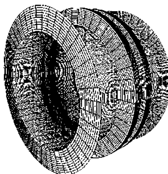
Figure 12: Description of 3D unsteady compressor model – Coupling of 3D Euler computations in blade-free volume. Multiple unsteady through flow solutions (tangentially uncoupled) in blade rows
