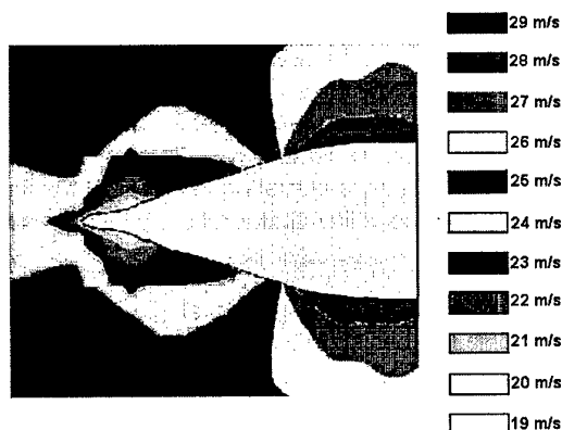
Fig. 6. Velocity distribution in the outer flow around the frontal part of the axisymmetric penguin body
