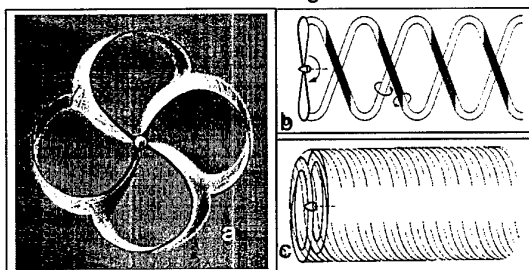
Fig. 31. Sketch of a "Bionic Ring Propeller" with 4 blades (a), while a usual propeller generates concentrated tip vortices (b), a continuous thin vortex sheet is shed from the trailing edge of the ring-like outer part of the Bionic Propeller (c)
