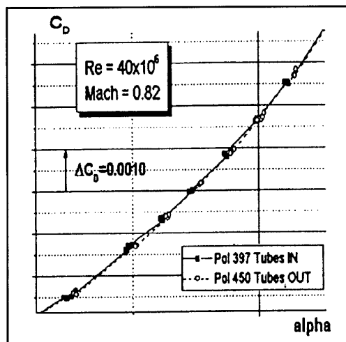
Figure 14: Measurement With and Without Pressure Equipment
