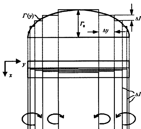
Fig. 23. Vortex model of a planar airfoil with finite span (redrawn after 49). Vorticity is shed from the trailing edge mainly in the wake of the tip region where the circulation distribution in the bound vortex shows the steepest gradient. At each side, the total circulation in the wake is equal to \Gamma_0 , the maximum circulation of the bound vortex (the roll-up mechanism is not shown in this graph.)
