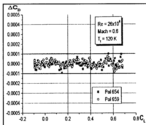
Figure 20: Short Term Repeatability of the Half Model Test Results
