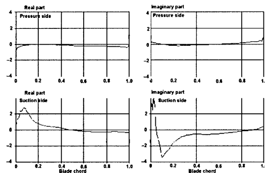
Figure 9: Unsteady Pressure Chordwise Distribution
