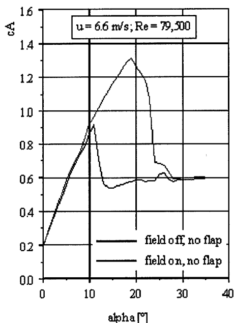
Fig. 22. Electro-aerodynamic separation control and super-circulation effect (low Reynolds number) [47]
