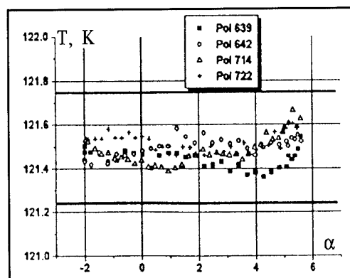
Figure 3: Temperature Stability
