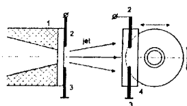
Fig. 2. Schematic of set up with discharge electrodes on ablated material: 1 - tetrazole, 2 - non-buffant min. nozzle, 3 - grounded central electrode, 4 - dielectric ablated working material
