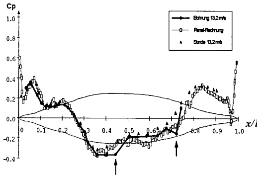
Fig. 4. Pressure distribution, experimental and numerical data
