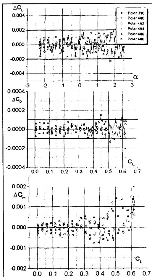
Figure 7: Deviation of Aerodynamic Coefficients
