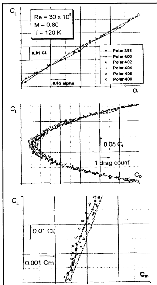
Figure 6: Selected Data Points of Repeatability Checks
