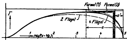
Fig. 30 Optimal circulation distribution at a propeller blade calculated by Betz [62]
