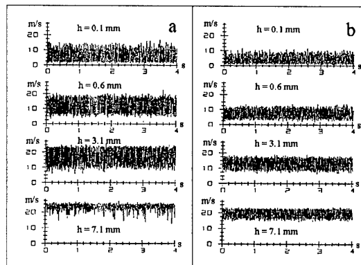
Fig. 9. Velocity fluctuations at the rear of the body (position: see arrow in Fig. 7). a (left side): without and b (right side) with turbulence generator; h distance from the body surface (from top to bottom: 0.1 mm, 0.6 mm, 3.1 mm, and 7.1 mm)
