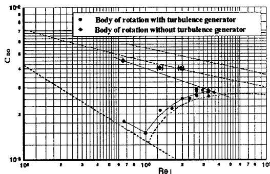
Fig. 3. Surface drag coefficients of the body of rotation plotted against Reynolds numbers. Note that in this graph Re was calculated by using the body length l as reference length. The two values in brackets should be neglected (artificial drag increase due to unfavourable Froude numbers in the test section). Dotted lines: laminar (below) and turbulent (above) flat plate. Dashed line on top: turbulent bodies with a length to thickness ratio of 4.2, cf. [31]
