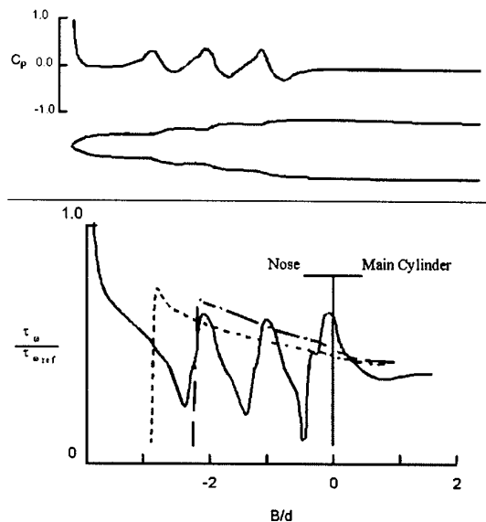
Fig. 12. Computed surface pressure distribution (above), and wall shear stress (below) in a three-stage nose body (solid line) compared with equivalent-area (dashed line) and equivalent-volume (chain line) half-elliptic noses (redrawn from [27])
