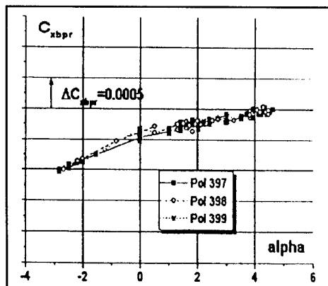
Figure 12: Repeatability of Base Pressure Measurement
