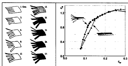
Fig. 25. a – Experimental optimization of a multiple winglet configuration, b – data of the initial and final wing tip v = 7 m/s, Re = 85\,000 , L = 3,9 (Experiments and graphs by M. Stache)
