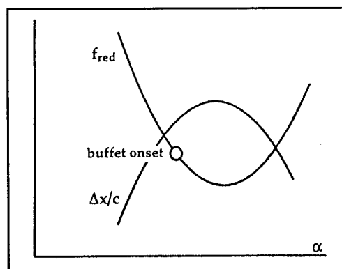
Figure 15: Buffet Onset Conditions
