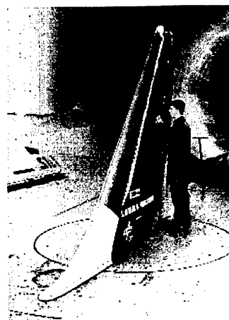
A320 Fin Model in ONERA S1MA
