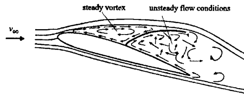
Fig. 20. Scheme of the flow pattern observed in smoke visualisation experiments. (PhD, G. Patone)
