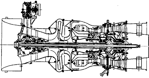
Advanced turboshaft engine
