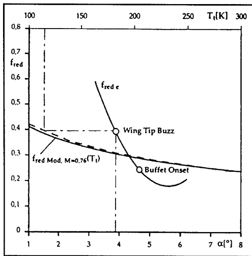
Figure 16: Reduced Frequency Behaviour
