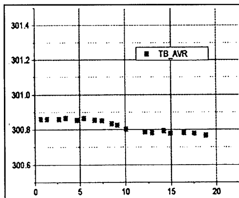
Figure 21: Half Model Balance Temperature Stability
