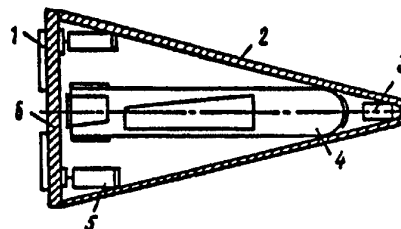
Fig. 2. The scheme of layout of a nose cone: 1 – bank control, 2 – heat-shielding body, 3 – explosive pusher for RA injection, 4 – RA with folded wings and control surfaces, 5 – explosive pushers for bottom separation, 6 – bottom.
