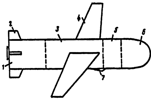
Fig. 3. The aerodynamic scheme and constituents of the winged RA: 1 – propulsion system, 2 – control surfaces, 3 – rescue means, 4 – wings, 5 – guidance system, 6 – supplementary reconnaissance means, 7 – air intake.
