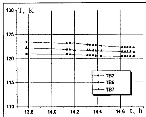
Figure 10: Temperature Stability of a Balance during a Test Run
