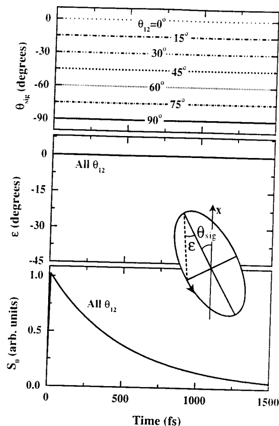
FIGURE 9.14. The temporal evolution of the azimuthal angle \theta_{sig}(t) , the ellipticity angle \epsilon(t) , and the total intensity S_0(t) of the TR-FWM emission for selected angles \theta_{12} between the two input polarizations, as calculated from the 2 \times 2 model of Section 9.5. This is an alternative representation of the TR-FWM simulations shown in Figure 9.13. For convenience the inset again shows the nomenclature and conventions that we adopt for defining the polarization ellipse.
