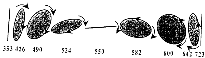
FIGURE 9.23. Schematic of the temporal evolution of the polarization ellipse for one beat period corresponding to the data in Figure 9.22 for \theta_{12} = 60^\circ .
