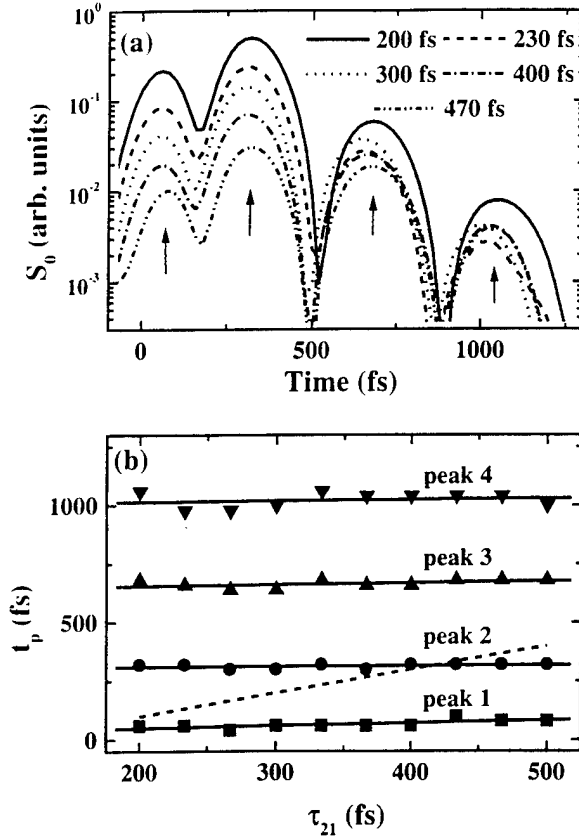
FIGURE 9.35. Results of measurements to distinguish quantum beating from polarization interference using two linearly x -polarized incident pump pulses: (a) Time-resolved measurements of the total intensity S_0 of the FWM signal for selected time delays \tau_{21} between two incident pulses, and (b) the time t_p at which each peak (indicated by an arrow in Figure 9.35(a)) occurs as a function of \tau_{21} , for a more complete set of time delays. The dotted line indicates a slope of unity.
