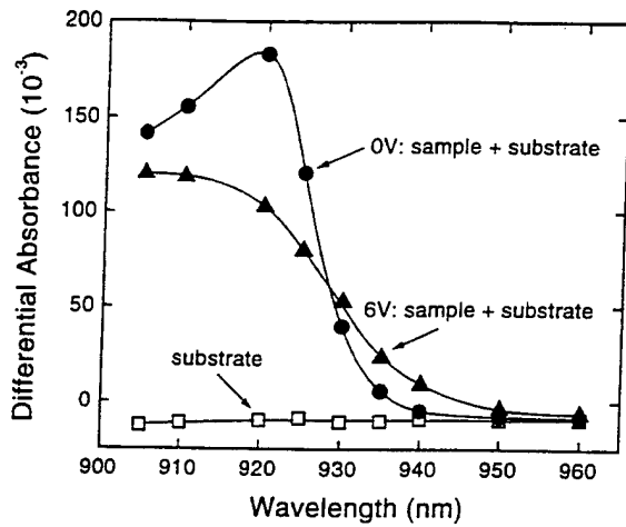
Fig. 4. Ellipsometric measurements of the differences in the absorbance of the MQW sample, including the substrate, for light polarized along the two principal crystallographic axes, \Delta\alpha_{MQWd} + \Delta\alpha_{sl} , for a bias of 0 V (solid circles) and 6 V (solid triangles) and of the substrate alone (open squares). The lines are guides to the eye.
