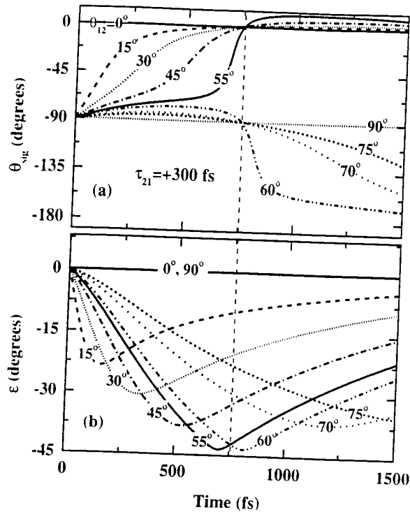
FIGURE 9.18. (a) The azimuthal angle \theta_{\text{sig}}(t) and (b) the ellipticity angle \epsilon(t) for selected angles \theta_{12} between the two input polarizations as calculated from the 2 \times 2 model modified to include EID, LFC, and BIF (see (9.20)). The time delay was fixed at \tau_{21} = +300 fs.
