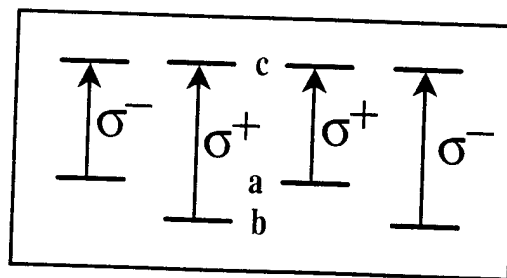
FIGURE 9.34. Schematic of four independent two-level systems for producing polarization interference.
