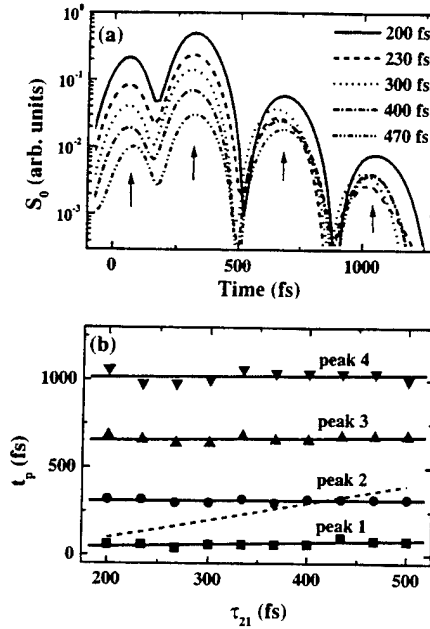
FIG. 3. Results of measurements to distinguish quantum beating from polarization interference using two linearly x-polarized incident pump pulses: (a) Time-resolved measurements of the total intensity S_0 of the FWM intensity for selected time delays \tau_{21} between two incident pulses, and (b) the time t_p at which each peak [indicated by an arrow in (a)] occurs as a function of \tau_{21} , for a more complete set of time delays. The dotted line indicates a slope of unity.
