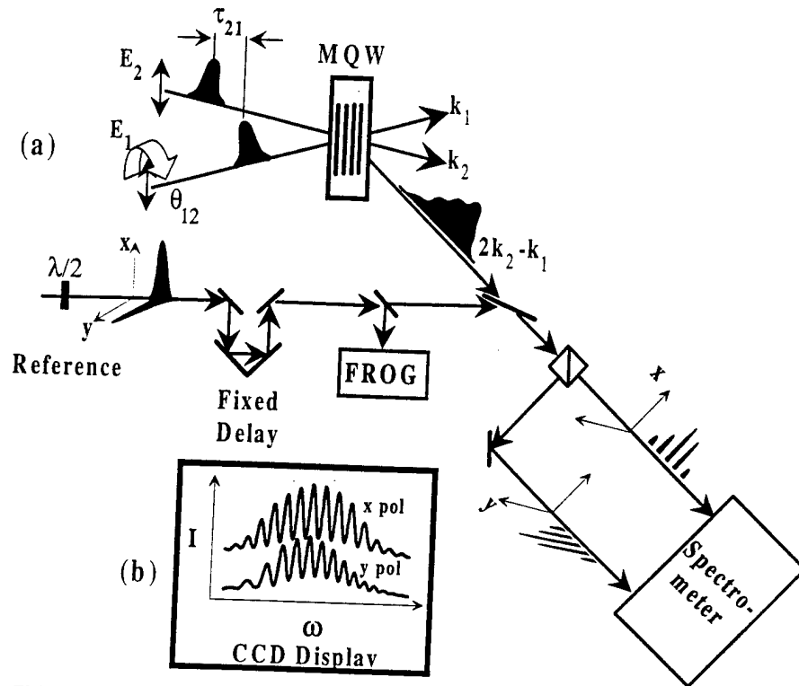
FIGURE 9.3. (a) Spectral interferometric geometry for the dual-channel (POLLIWOG) measurement of the amplitude, phase, and polarization state of the FWM signal; (b) schematic of spectral interferograms for the x and y components as displayed on the CCD array attached to the spectrometer. FROG denotes the setup for the characterization of the reference pulse by frequency-resolved optical gating.
