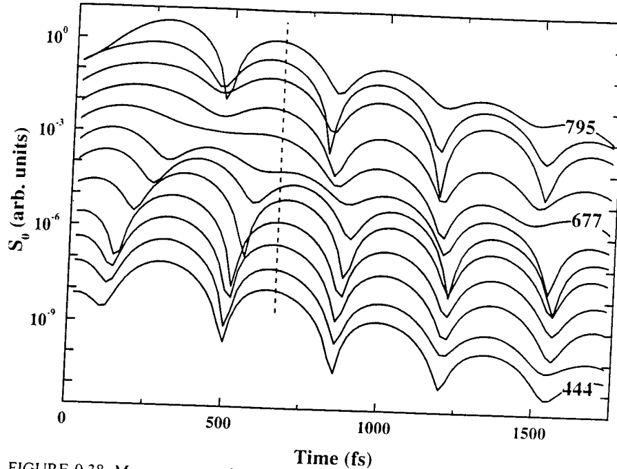
FIGURE 9.38. Measurements of the total intensity S_0 of the FWM signal as a function of time for equally spaced time delays \tau_{21} between the two incident pulses in the range between 444 and 795 fs.
