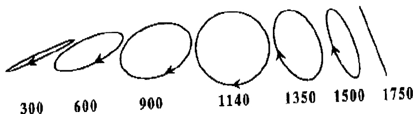
FIGURE 9.8. Schematic drawings of the polarization ellipses corresponding to the data in Figure 9.7 for selected time delays that illustrate the origin of the discontinuity in the orientation of the polarization ellipse shown in Figure 9.6.
