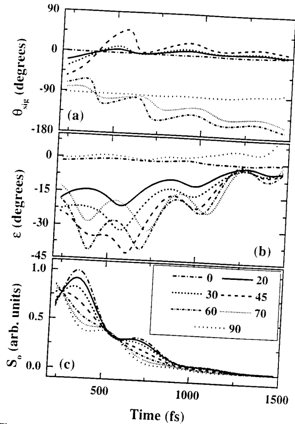
FIGURE 9.31. The measured time-resolved (a) azimuthal angle \theta_{\text{sig}} , (b) ellipticity angle \epsilon , and (c) total intensity S_0 in the weak quantum beat regime, corresponding to the data of Figure 9.30.
