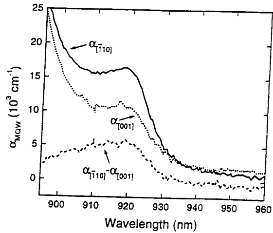
Fig. 1. The measured linear absorption coefficients of [110]-oriented \text{In}_{0.13}\text{Ga}_{0.87}\text{As} -GaAs MQW's as a function of wavelength for incident light polarized parallel to the [\bar{1}10] (solid line) and [001] (short dashed line) crystallographic axes of the [110]-oriented GaAs-InGaAs MQW's, and the difference in the two coefficients (long dashed line).
