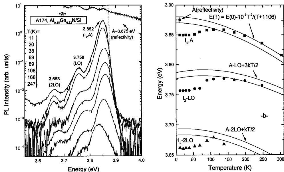
Fig. 2. a) Photoluminescence and reflectivity (11 K) spectra of Al_{0.18}Ga_{0.82}N/Si . b) Temperature dependence of luminescence energies in Al_{0.18}Ga_{0.82}N/Si . Two parallel solid lines separated by 10 meV correspond to the \pm 5 meV uncertainty in the energy of the A-excitonic gap
