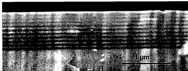
Fig. 3. SEM cross-section view of a ten-period Al_{0.2}Ga_{0.8}N/AlN Bragg mirror on (111)Si
