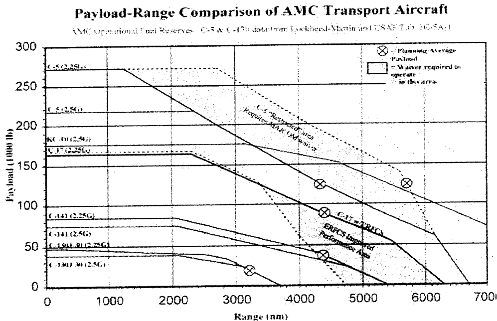
FIGURE 6. AMC AIRCRAFT PAYLOAD-RANGE COMPARISON
