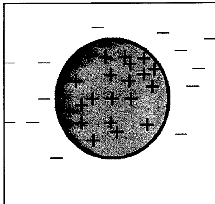
Figure 9: quadrupole moment.
