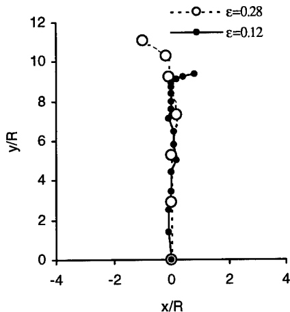
Fig 9. Trajectories of two eddies (with different \epsilon ) from the moment t = 0 . For comparison with similar data calculated in [4], non-dimensional coordinates ( x/R , y/R ) and non-dimensional time ( \Omega t ) are used. The non-dimensional time interval between two nearest points (for the same eddy) is equal to 20
