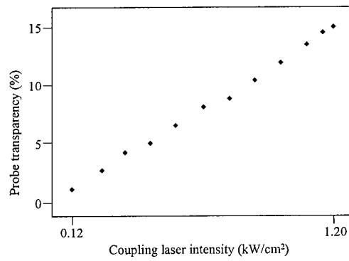
FIG. 17. Probe transparency versus coupling laser intensity.
