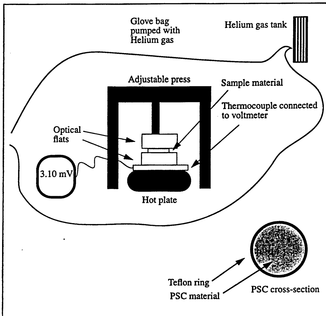
Figure 8. An adjustable press for producing concavity-free samples of PSC.
