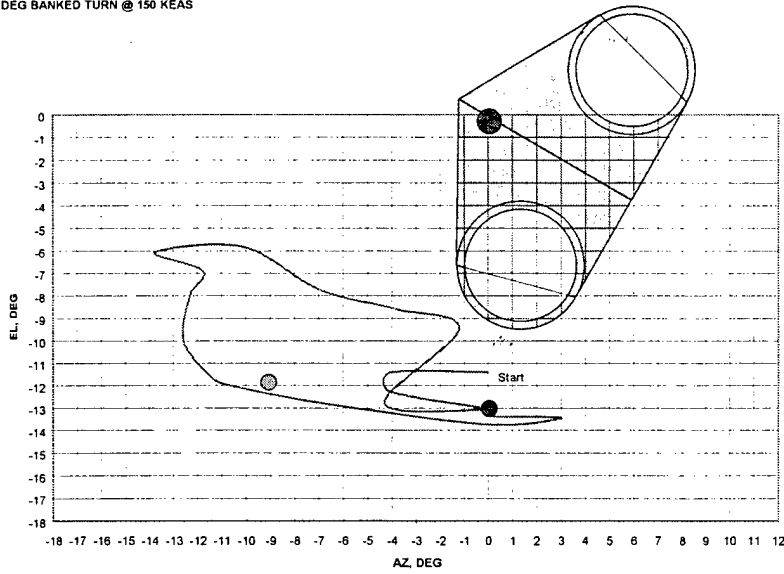
TOW CABLE AZ & EL AT A/C 60 DEG BANKED TURN @ 150 KEAS
