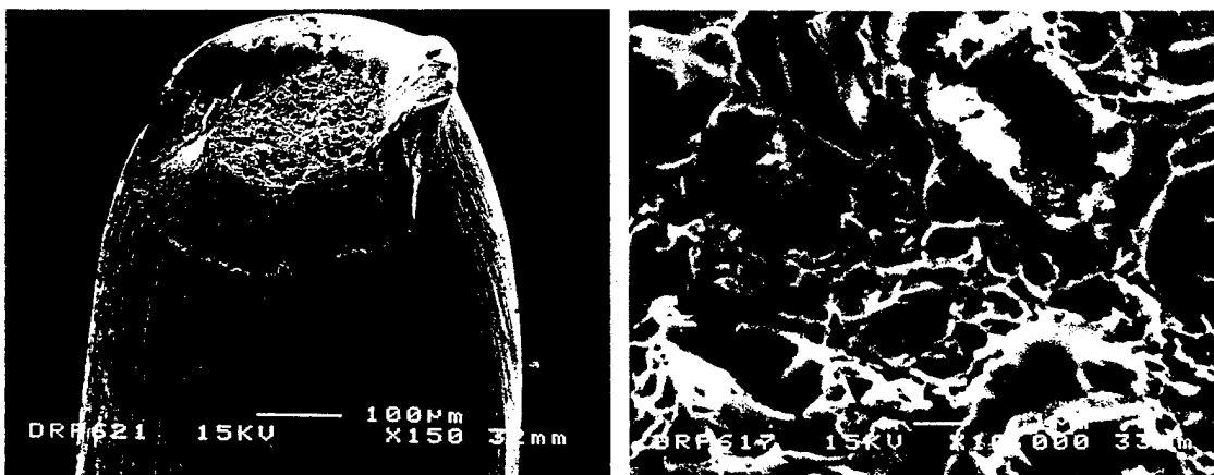
Figure 8. Fractured wires from cable A tensile test.
