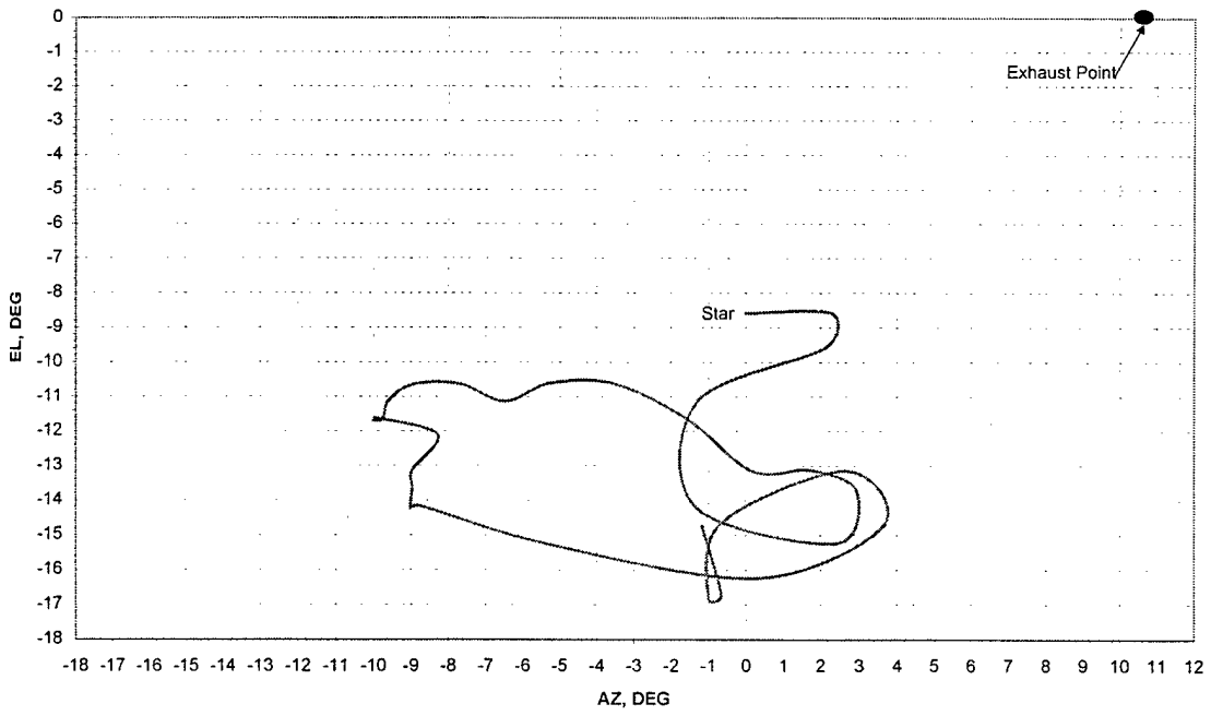
TOW CABLE AZ & EL AT A/C 60 DEG BANKED TURN @ 200 KEAS
