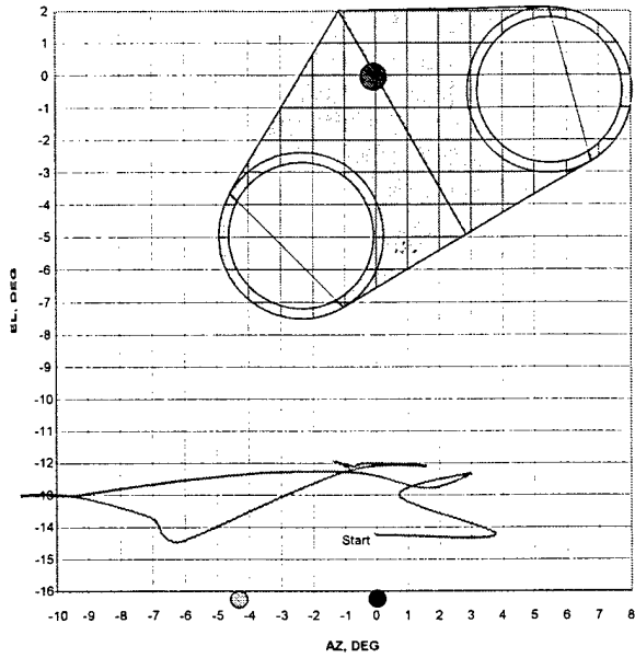
Figure 12. Cable position at the exhaust plane as predicted by CBAS for 30 0 AoB at 120KEAS.
