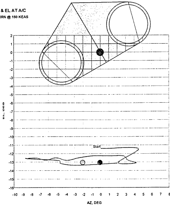
Figure 13. Cable position at the exhaust plane as predicted by CBAS for 30 0 AoB at 150KEAS.
