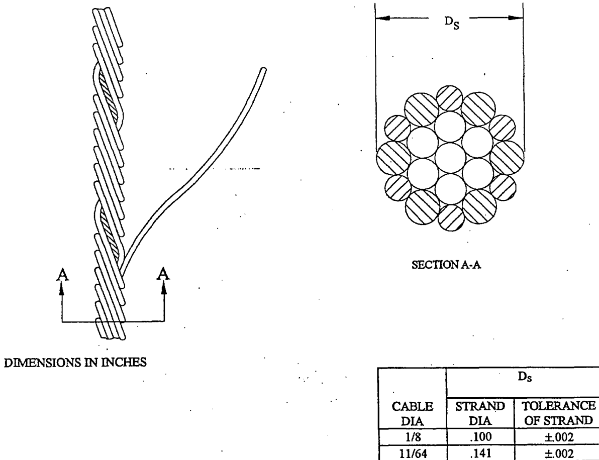
FIGURE 1. Strand Construction
