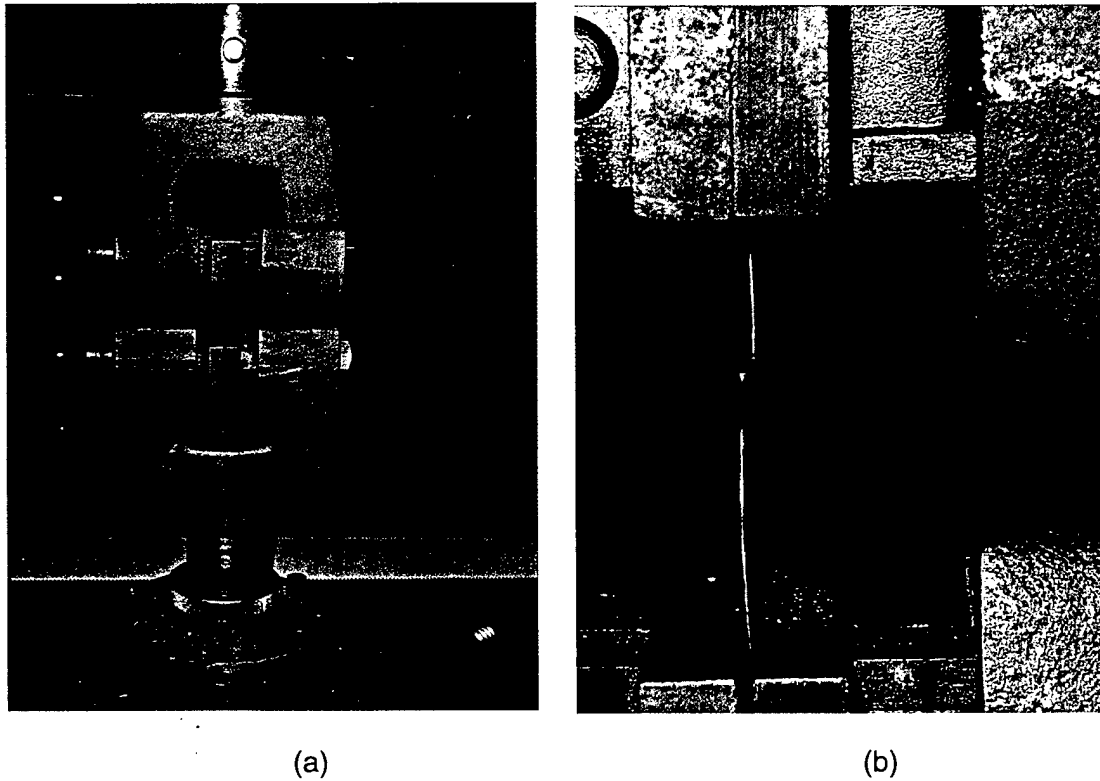
Figure 16. Tensile test of individual wires.
