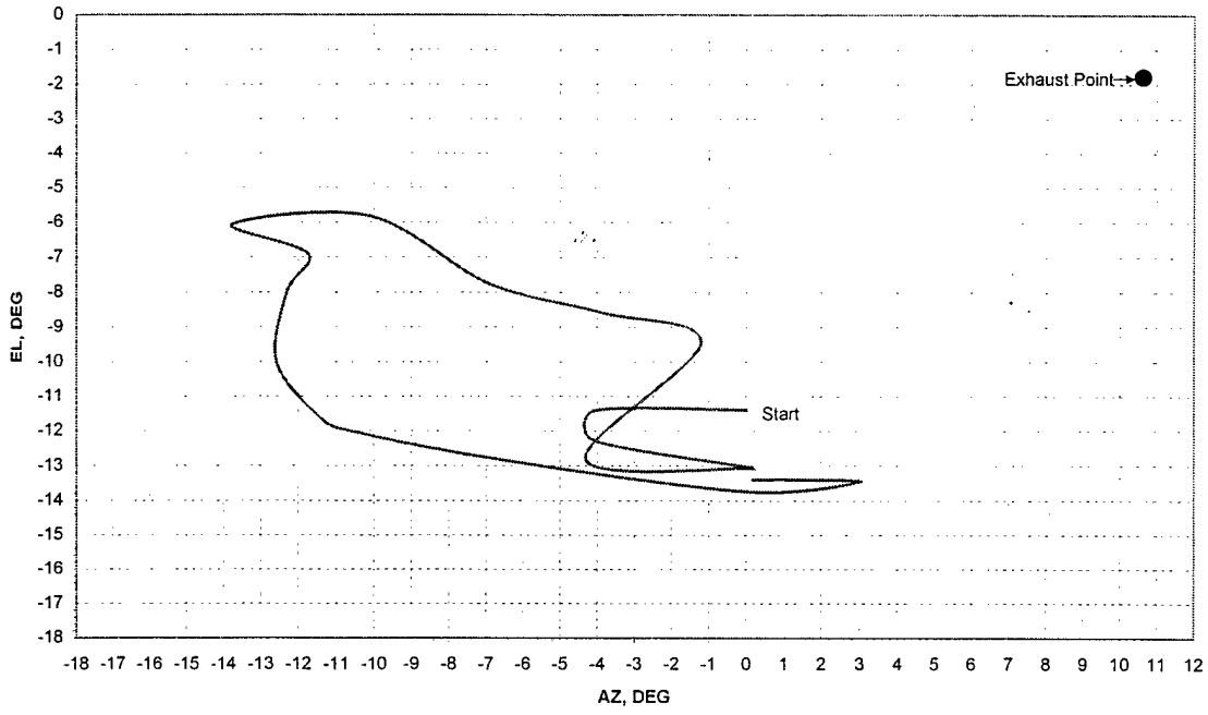
TOW CABLE AZ & EL AT A/C 60 DEG BANKED TURN @ 150 KEAS
