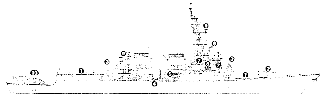
Figure 7: Scaled drawing of the Oscar Austin destroyer [From Ref.30].
