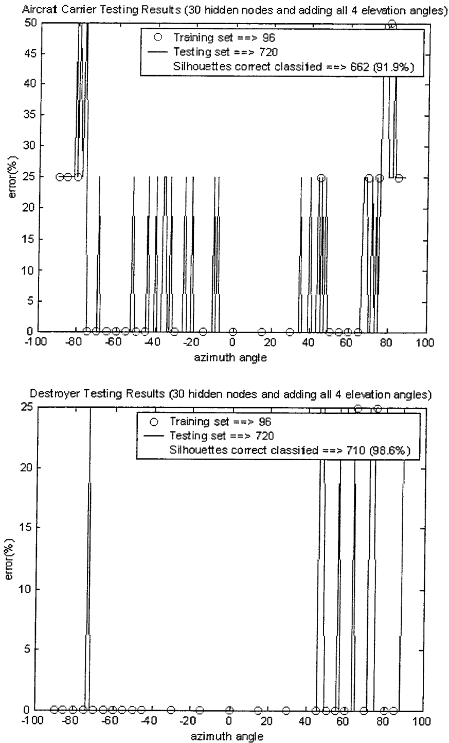
Figure 33: Accuracy with respect to azimuth for aircraft carrier and destroyer
