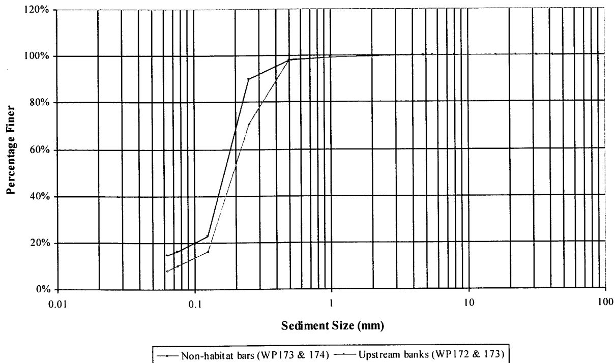
Figure A36: Fort Peck Reach - Comparison of non-habitat bars in Sampling Reach 14 with potential upstream bank sources of sediment
