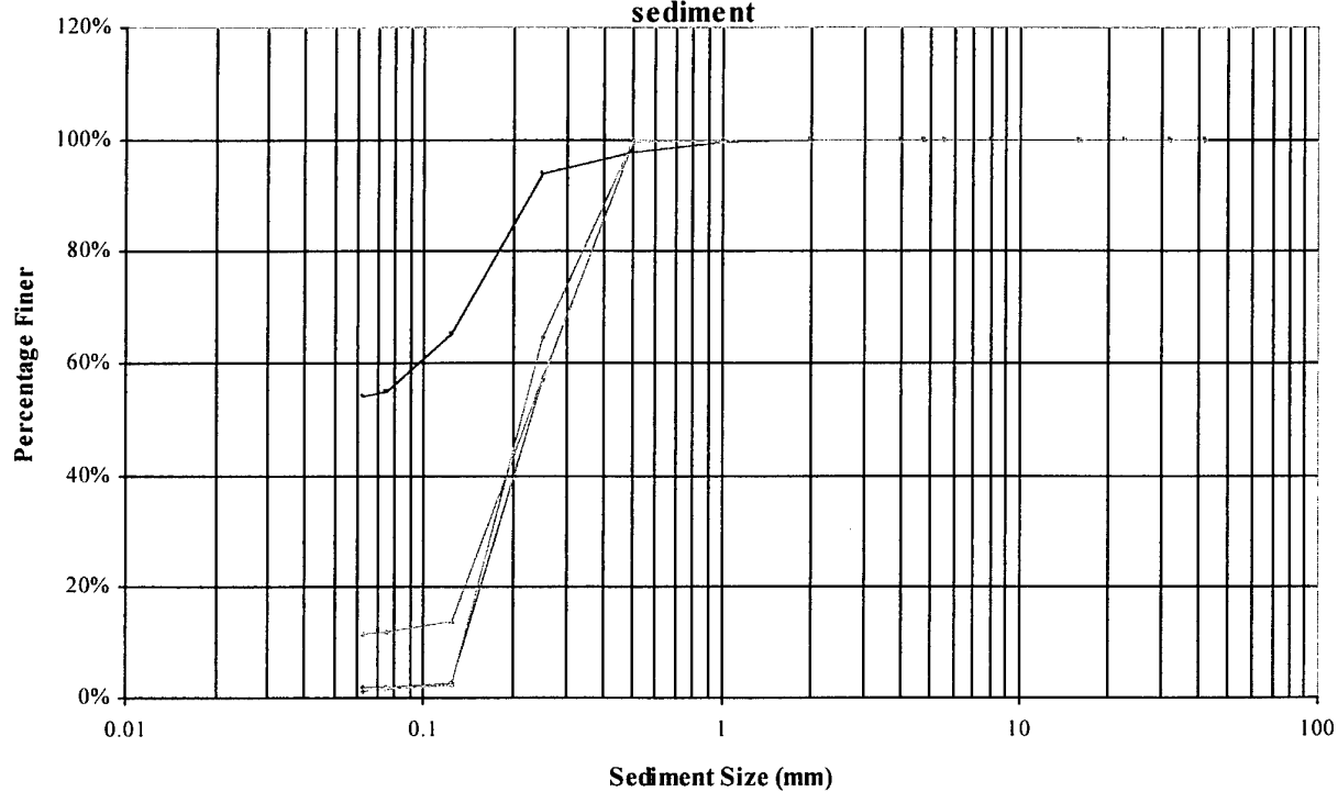
Figure A21: Fort Peck Reach - Second comparison of a habitat bar and a non-habitat bar in Sampling Reach 8 with potential upstream bank and tributary sources of sediment
