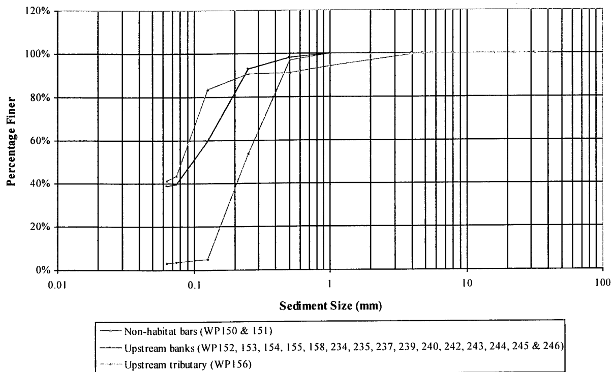
Figure A30: Fort Peck Reach - Comparison of non-habitat bars in Sampling Reach 12 with potential upstream bank and tributary sources of sediment in Geomorphically Similar Reach 6
