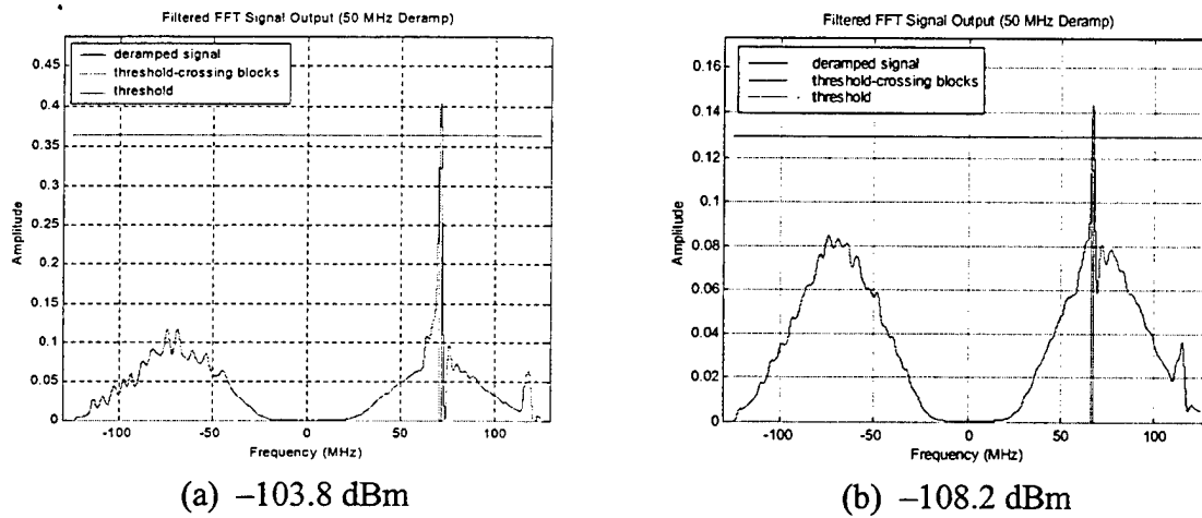
Figure 5.9 Deramped Output of Weak Signals
