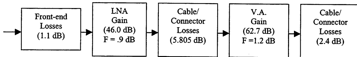
Figure 3.21 Noise Figure Block Diagram
