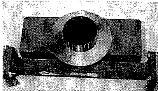
Figure 3.7 HP X375A Variable Attenuator
