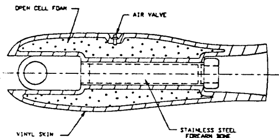
Figure 13. Typical Segment Skin Construction
