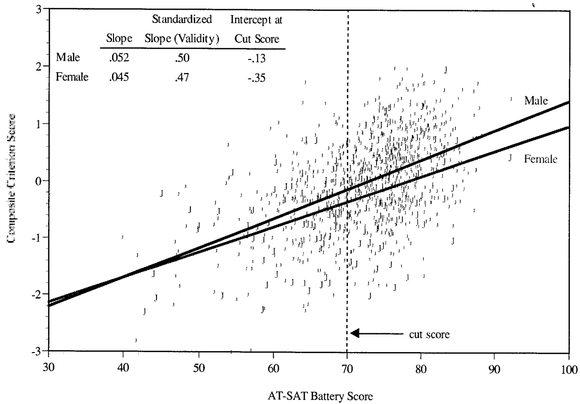
Figure 5.6.3. Fairness Regression for Females Using AT-SAT Battery Score and Composite Criterion
