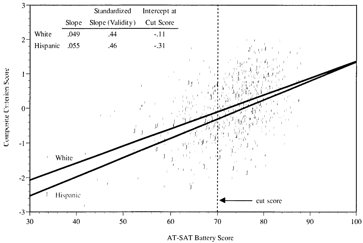
Figure 5.6.2. Fairness Regression for Hispanics Using AT-SAT Battery Score and Composite Criterion
