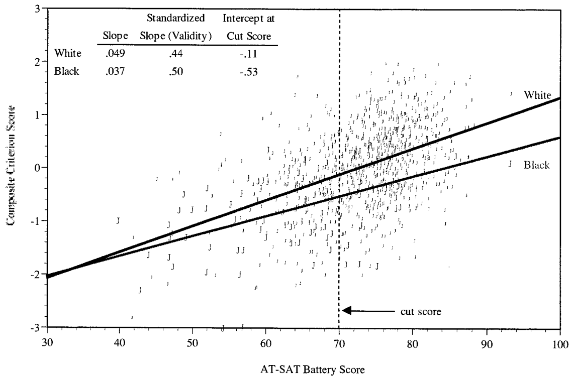
Figure 5.6.1. Fairness Regression for Blacks Using AT-SAT Battery Score and Composite Criterion
