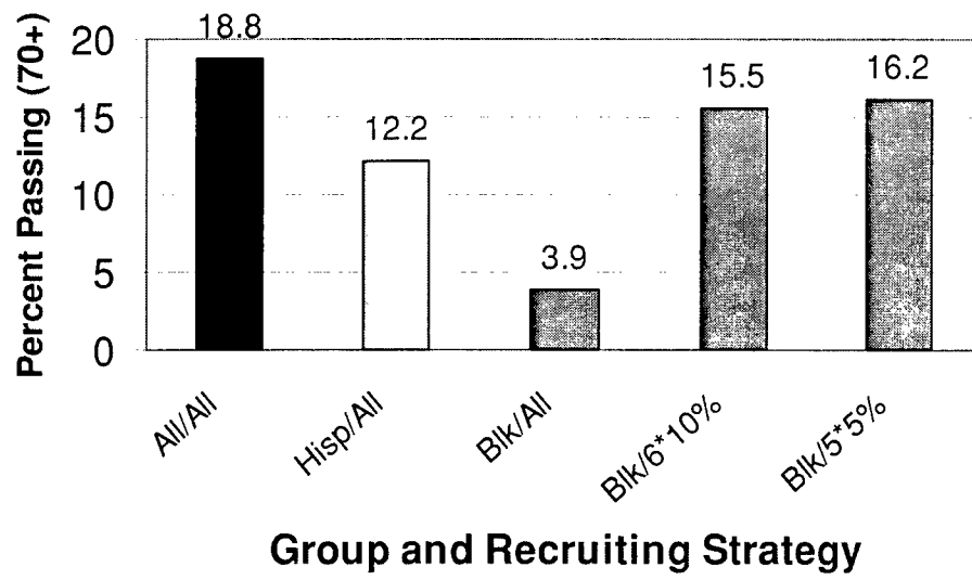
Figure 5.6.6. Percent Passing by Recruitment Strategy
