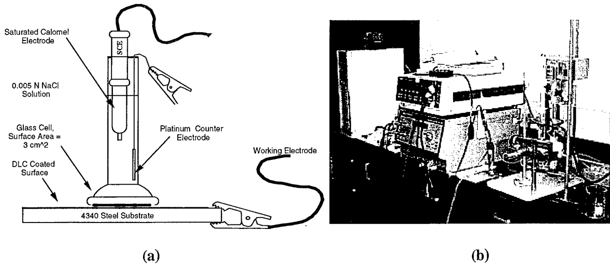
Figure 1. Schematic of the (a) Corrosion Cell and (b) Potentiostat and FRA Used in Experiment.
