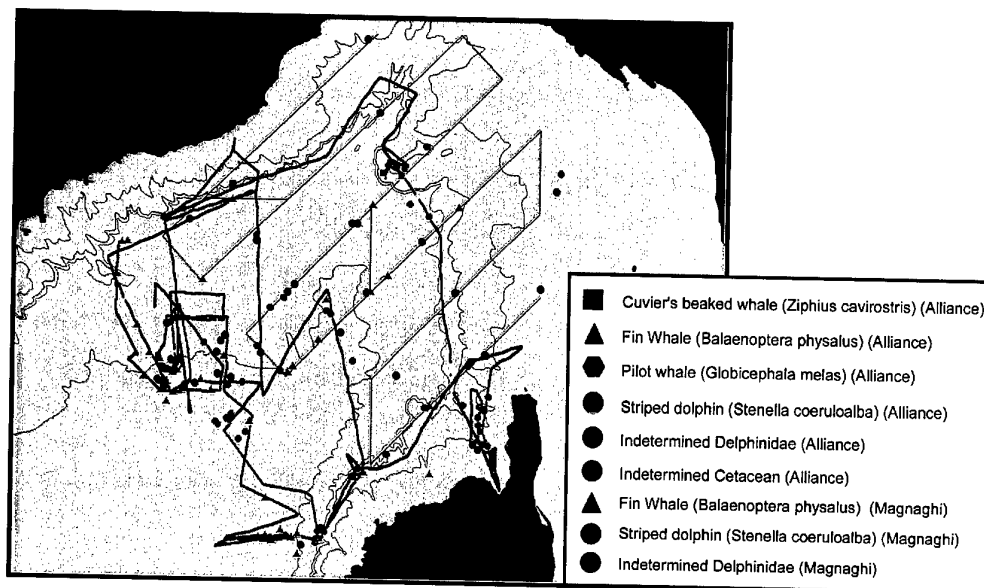
Figure 06-C.1 Sirena 99 cruise. Alliance conducted acoustic and visual measurements along the track shown in black. The Italian Navy Hydrographic vessel Magnaghi conducted oceanographic and prey field measurements along the track shown in green. The symbols show the visual sighting of the cetaceans by both vessels.
