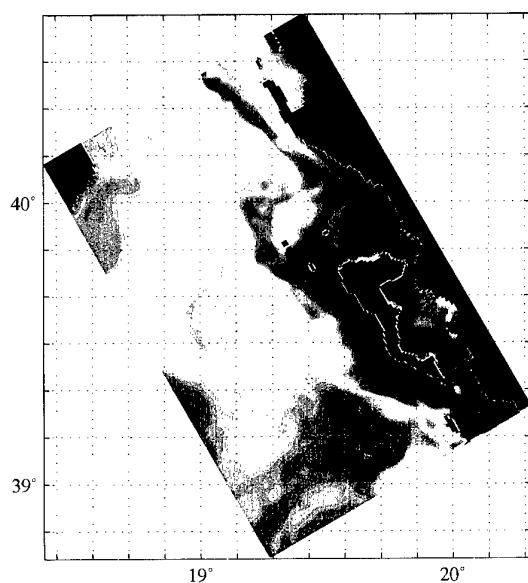
Figure 01-A.4. Forecast of surface temperature for 11 September 1999, 12 days after model setup during CORFU99. The temperature ranges from 16 to 28^{\circ} C. Upwelling of cold water off the coasts of Albania and Corfu is a consequence of atmospheric forcing.
