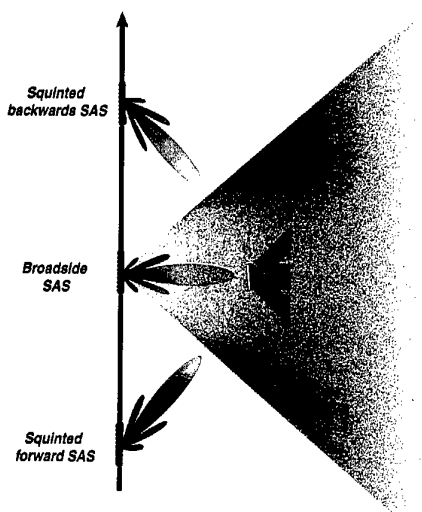
Figure 03-B.3 Geometry of the multi-aspect synthetic aperture sonar.
