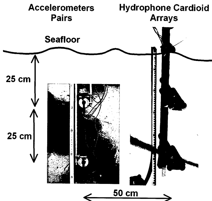
Figure 03-D.1 Sensor hydrophone array.
