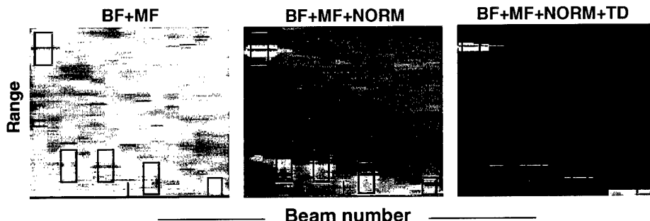
Figure 04-A.9 Unnormalized Range-Bearing sonar image generated from the receive signal amplitudes of each beam (left), the same data set after normalization (middle), the same data set after thresholding (right). Rectangles are 1 \times 1 km. This series of displays allows an operator to classify alarms by reviewing the normalized/unnormalized sonar displays to determine if a contact could be due to e.g., a reverberation edge, similar to the bottom four contacts in the right hand image.
