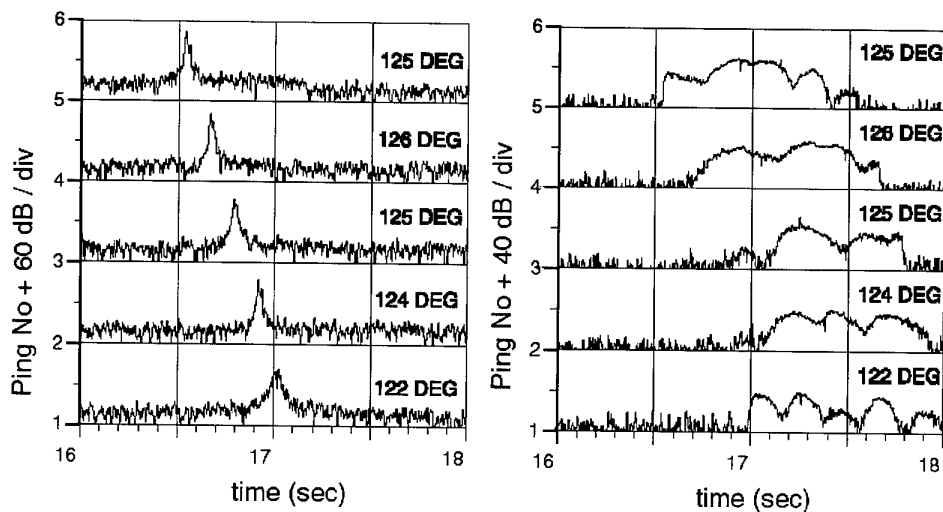
Figure 04-B.3 A zoom view of echo signals shows that multipath effects come and go from ping to ping.
