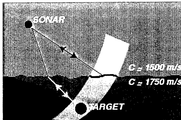
Figure 03-A.1 Geometry of a buried mine sonar.
