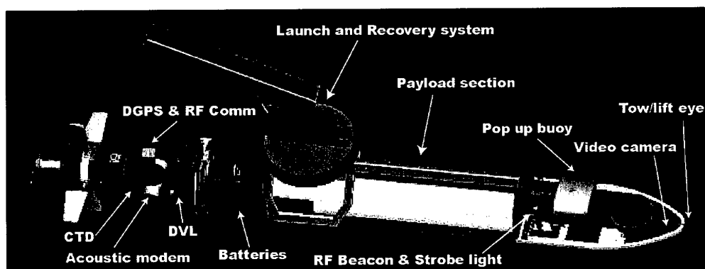
Figure 01-B.11 Detail Of the Ocean Explorer AUV.
