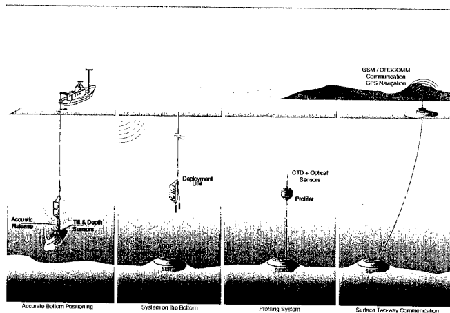
Figure 01-A.8. The Environmental Profiler in Trawl-safe, Real-time configuration (SEPTR) is a high value multi-sensor platform for REA in accessible areas. After deployment, it does not interfere with fishing activity. At preprogrammed times, a float rises for measurements in the water column and data delivery.
