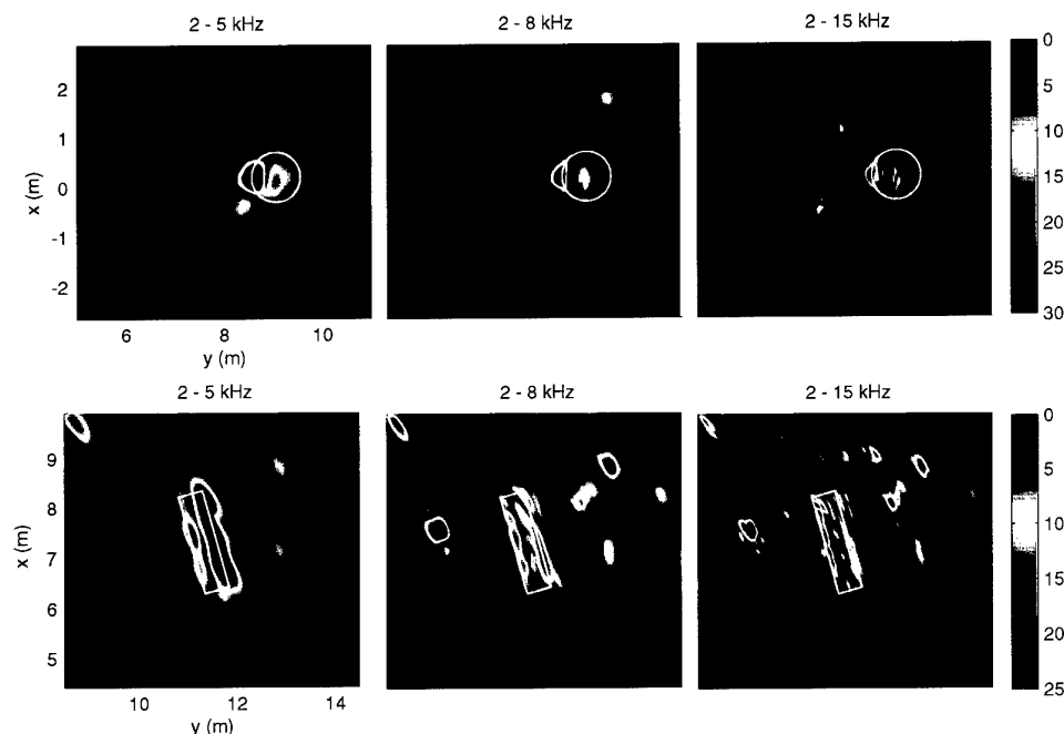
Figure 03-A.4 High resolution images of buried sphere and cylinder.
