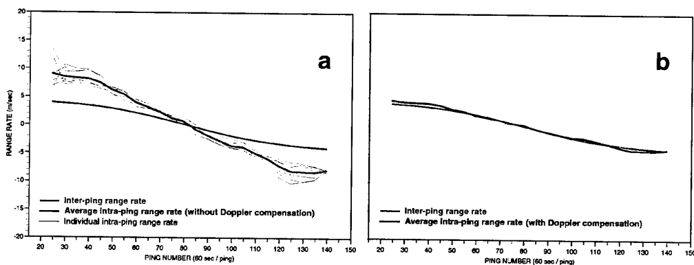
Figure 04-A.7 Comparison between inter-ping (red) and intra-ping range rate estimation without (Fig. 4-A.7a) and with (Fig. 04-A.7b) Doppler compensation. Range rate estimation from sub band delay time measurements within one ping is feasible, but requires a Doppler-independent correction factor.
