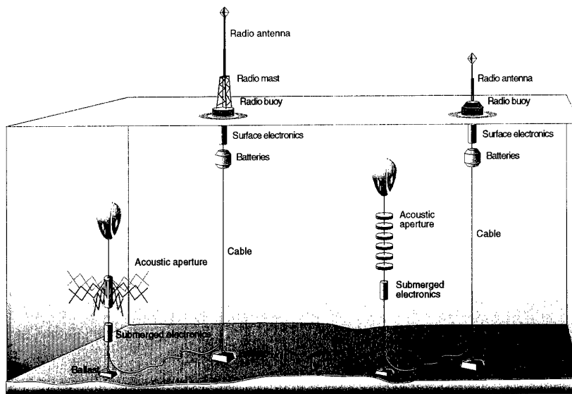
Figure 04-B.10 New DUSS prototype. deployable receiver and transmitter units.
