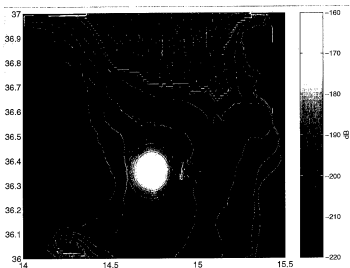
Figure 04-D.5 Model predictions of monostatic reverberation versus azimuth for rough sediment scattering on the Malta Plateau. The predictions do not show the strong variability with azimuth visible in the dataset.
