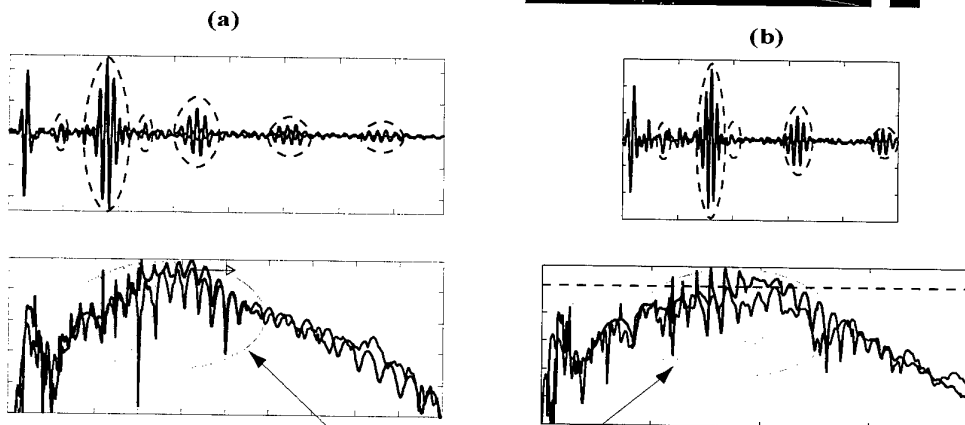
Figure. 03-A.10 GOATS 98 data-model comparison of time and frequency response of 1 m \varnothing air-filled sphere in free space (a) and flush buried (b). The model assumes the sphere in the free field even when buried. Main results of elastic wave analysis are included.
