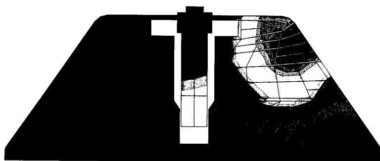
Figure 03-E.5 Colour contours show displacement magnitude on a plane that bisects the mine.
