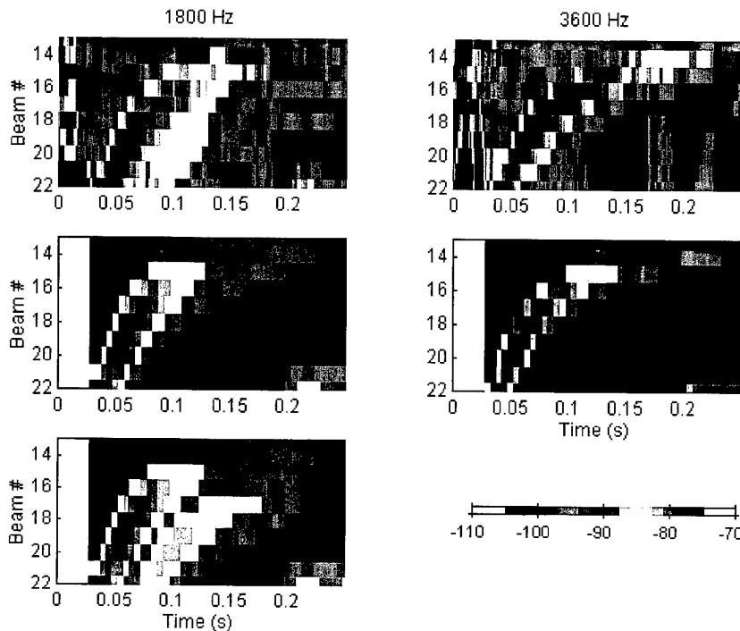
Figure 04-C.1 Comparison of measured data at: a) 1800 Hz and b) 3600 Hz with modelled results for water-sediment interface scattering c) 1800 Hz, d) 3600 Hz and e) 1800 Hz modelled results with water-sediment interface scattering and interface scattering at 25 m sub-bottom. The lettering sequence follows a left to right, top to bottom order. The quantity plotted is received level minus source level.
