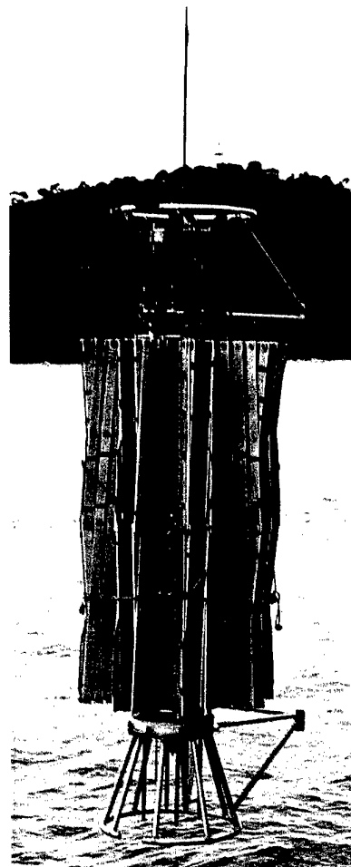
Figure 04-B.10 New DUSS prototype. deployable receiver and transmitter units.
