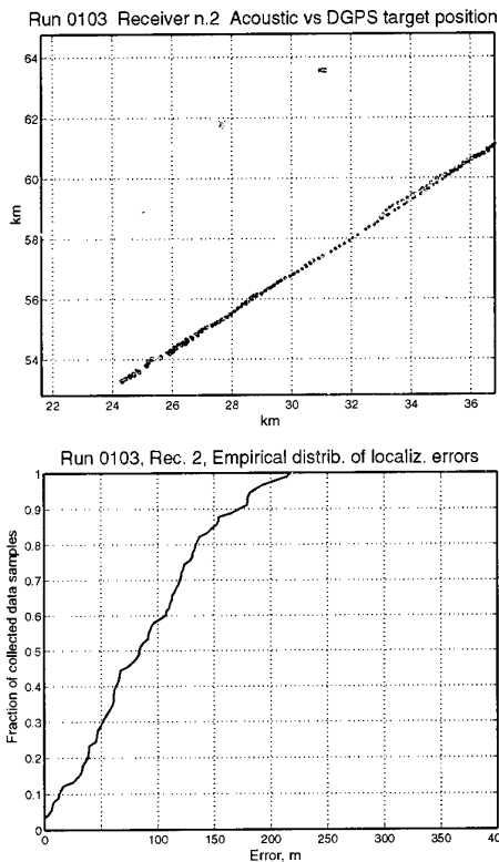
Figure 04-B.6 Contact localization consistency of DUSS networks was analyzed as a function of system characteristics.
