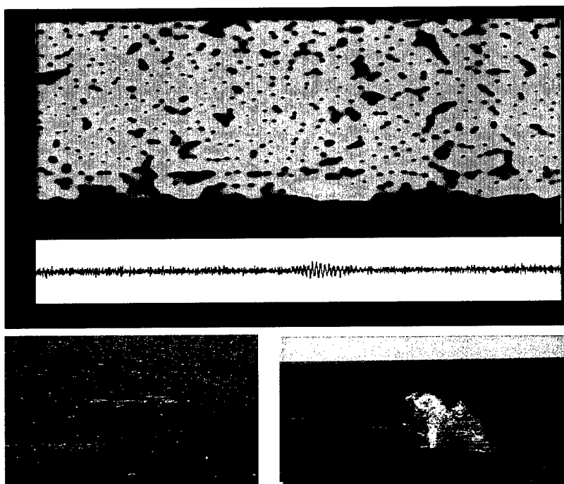
Figure 06-C.3 A one second, 25 Hz - 18 Hz low frequency, down sweep signal from a fin whale. Photographs show visual sightings.
