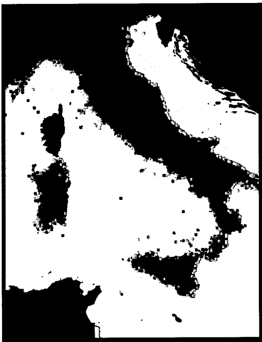
Figure 06-C.7 Location of cetaceans (see key) stranded along the Italian coast 1986-1996.
