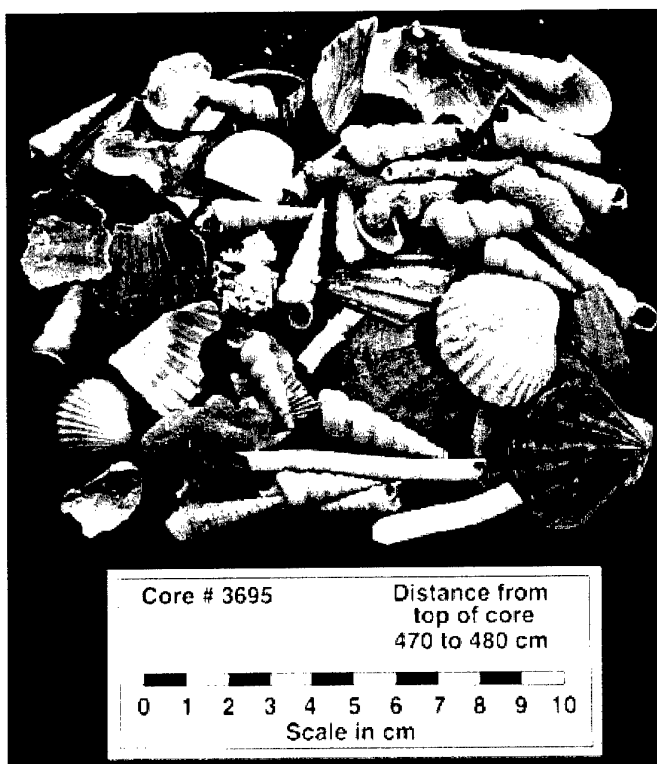
Figure 04-C.3 Shell material corresponding to high-speed layer in Figure 04-C.2 near 5 m depth sub-bottom.
