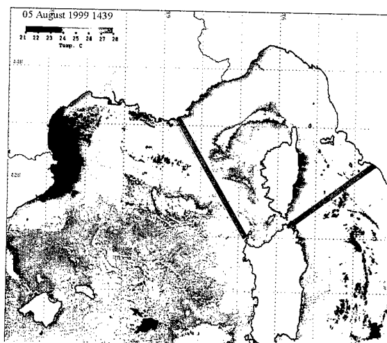
Figure 06-C.2 Representative sea surface temperature during the Sirena 99 cruise period (5 August 1999). Red lines outline the boundary of the Ligurian Sea Cetacean Sanctuary.
