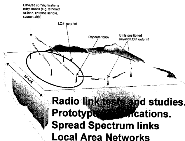
Figure 04-B.8 Radio network techniques implement the "sonar Internet" of DUSS units for experiments.
