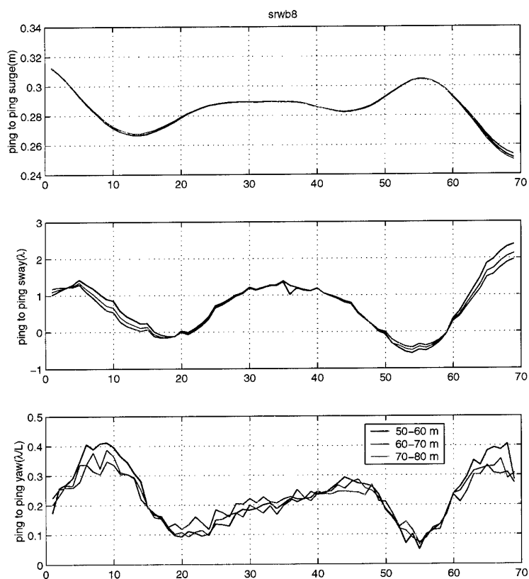
Figure 03-B.5 DPCA micronavigation of MASAI'99 (carrier frequency 100 kHz, 20 kHz bandwidth, 128 channels spaced at 1/2 ) for three different ranges giving three independent estimates of the motion in the slant-range plane. The yaw estimate is biased, possibly because of calibration errors of the physical array.
