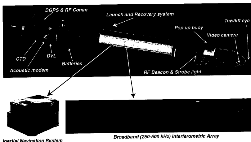
Figure 03-B.6 The MCM autonomous underwater vehicle consists of a propulsion section which houses the common navigation components, a payload sections with the INS and the interferometric wide band sonar and a nose cone section with a video camera and a recovery line system.
