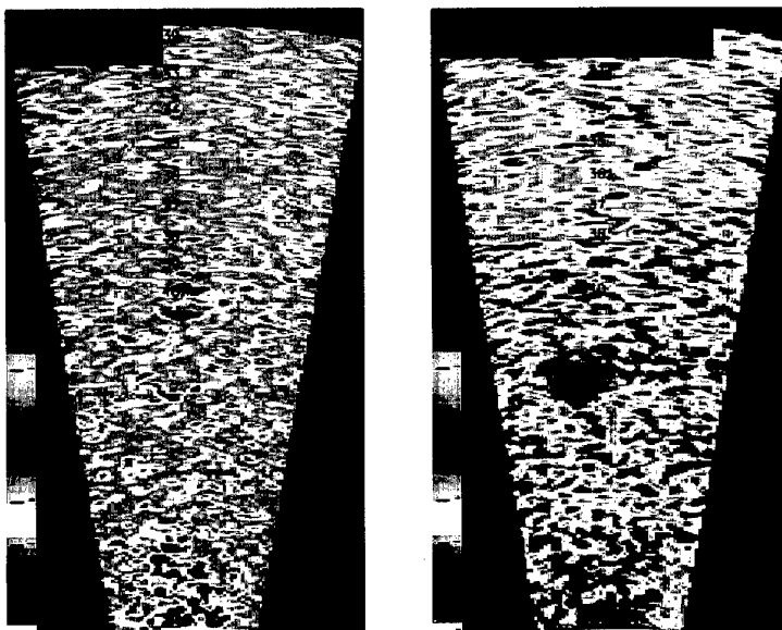
Figure O3-D.3 Scattering strength versus range and azimuth at 140 kHz for a hard, rough bottom (left) and a soft, inhomogeneous bottom (right).
