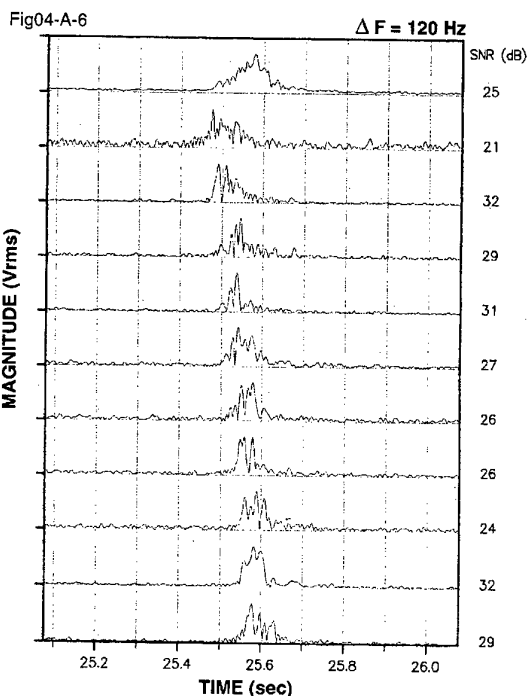
Figure 04-A.6 Normalized intra-ping sub band echoes signals with SNR estimates for each sub-band indicated on the right of each signal. The differential time delay between the sub-bands is shown. The top plot represents the normalized average of the individual outputs. Note that the echoes from different sub bands are uncorrelated. SNR differences of up to 10 dB, the Doppler-induced differential delays and the relatively low SNR of the sum signal (top of this figure) suggest detector schemes different from simple averaging.
