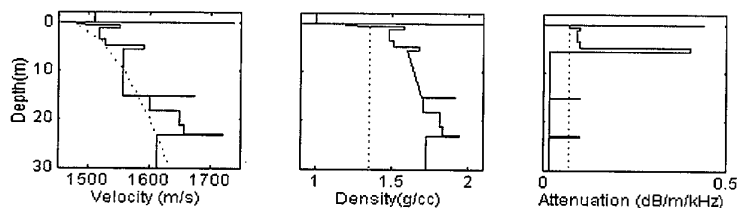
Figure 04-C.2 Site S sediment parameters. Parameters from Holland and Osler (1998) (solid line) and that used in the model predictions of Figure 04-C.1 (dotted line).
