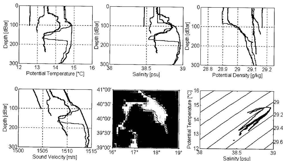
Figure 01-A.2. Temperature, salinity, density anomaly and sound velocity profiles truncated at 300 m depth. The cold and least saline coastal water is denser than intermediate water further out. In the temperature-salinity diagram, it appears as a dot on the same isopycnal as the Eastern Mediterranean Deep Water.
