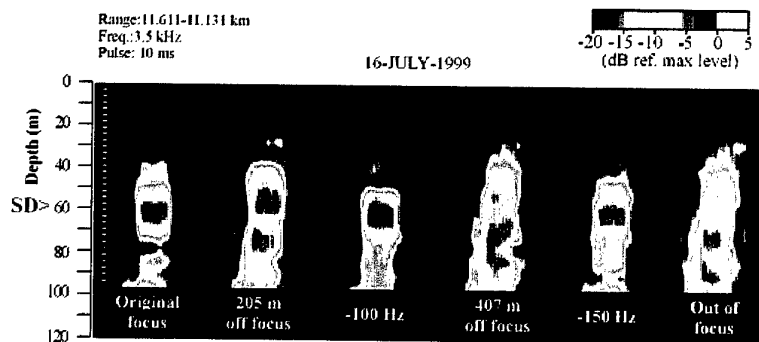
Figure 06-B.6 Frequency shifting for refocusing.
