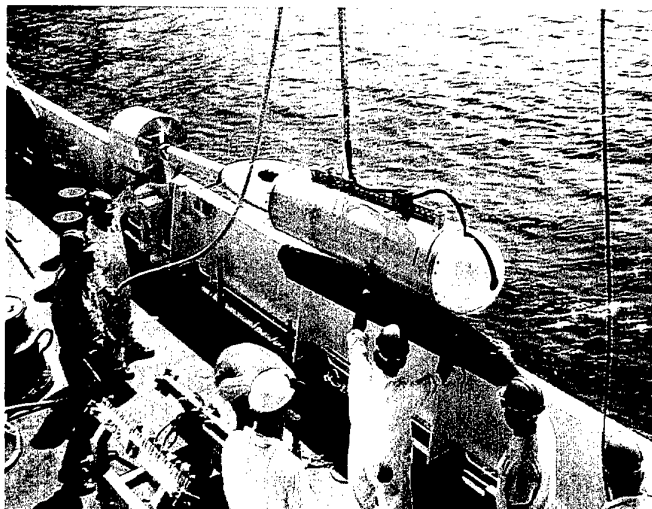
Figure 03-B.2 The 100 kHz programmable sonar deployed from R/V Alliance in June 99 during the MASAI'99.
