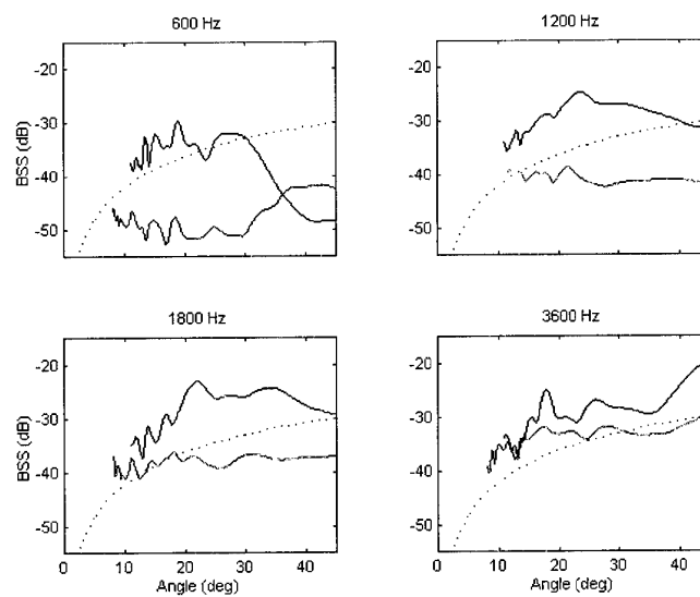
Figure 04-C.4 Scattering strength results at two sites: silty clay with interstitial sandy layers (red) and sandy with thin silt layer at interface (blue). Also shown is the NATO standard (dotted line).
