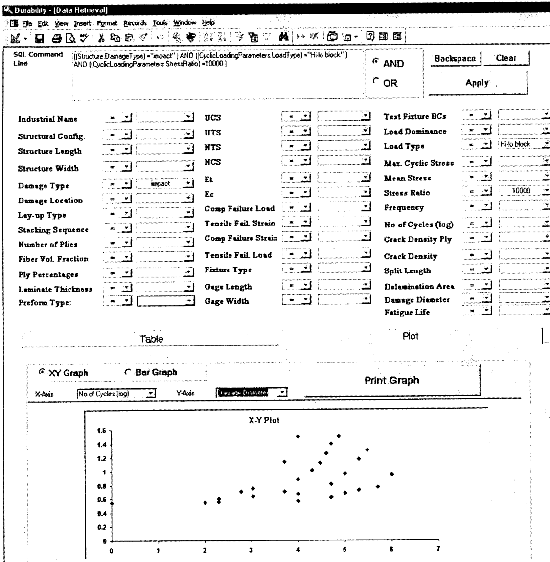
FIGURE 33. NUMBER OF CYCLES (LOG) VS DAMAGE DIAMETER FOR IMPACTED SPECIMENS UNDER COMPRESSION DOMINATED BLOCK LOADING
