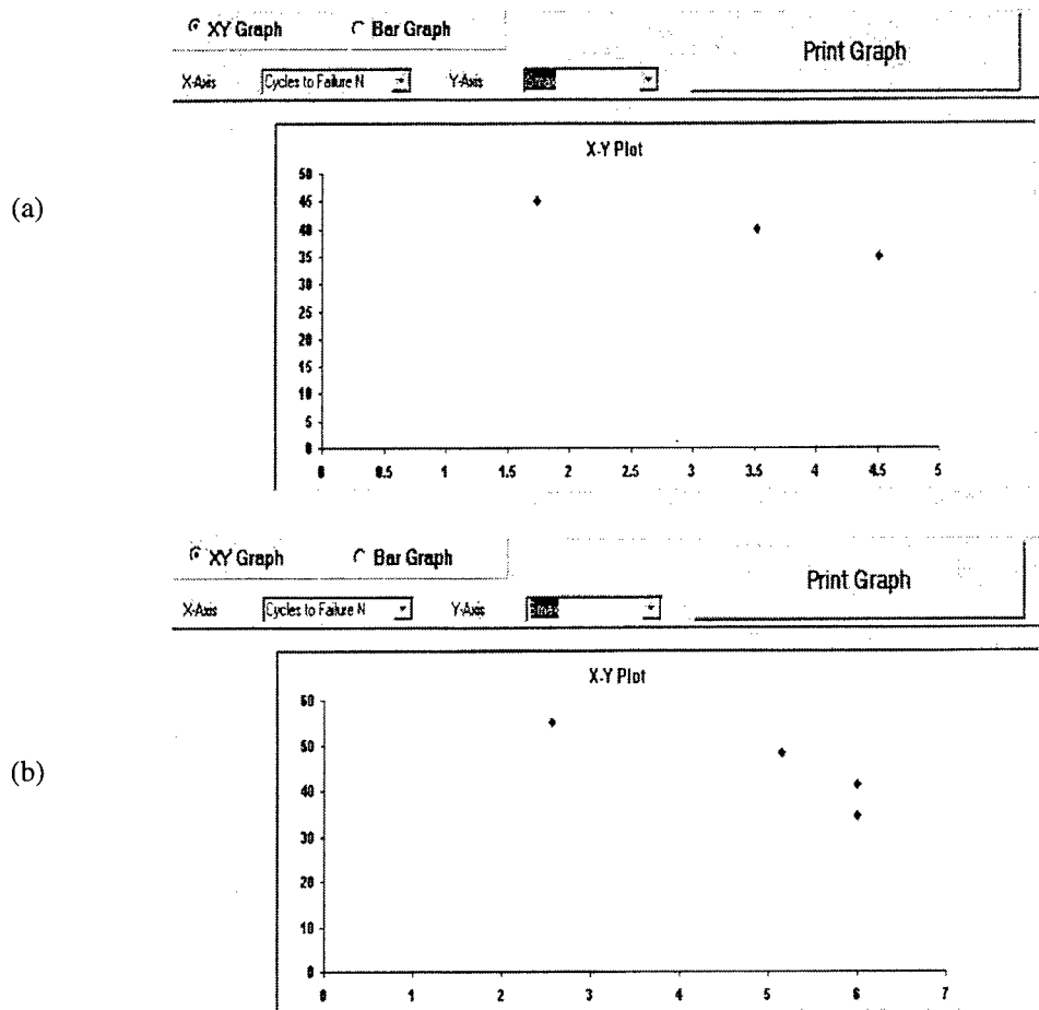
FIGURE 35. S-N CURVES FOR (a) OPEN HOLE AND (b) IMPACTED COMPOSITE COUPONS UNDER CONSTANT AMPLITUDE C-C LOADING
