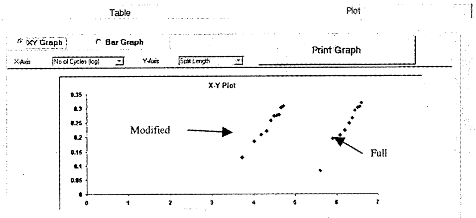
FIGURE 30. COMPARISON OF GROWTH IN SPLIT LENGTH DAMAGE METRIC UNDER FULL AND MODIFIED TWIST FATIGURE LOADING SPECTRUM
