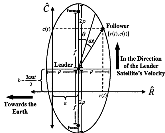
Figure 51 General Follower Orbit in the R/C Plane
