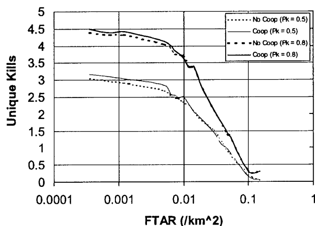
Figure 5.1 Unique Kills Sensitivity to FTAR for 2 Warheads
