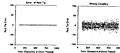
Figure 6. The error between the actual and predicted dynamics of the rod at the tip for weak coupling (left) and strong coupling (right).
