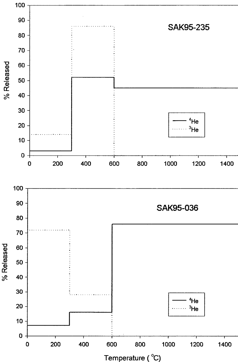
Figure 2.2 Release pattern of 3 He and 4 He during the 300°, 600° and 1500° heating steps of sample SAK95-036 and 235. Other samples show similar patterns. 100 percent of the cosmogenic 3 He is released in the 300° and 600°C heating steps. In contrast, only a few percent of the 4 He is released in the first step and almost 50 to 80 percent of the 4 He is released in the last step. The 3 He/ 4 He of the last step characterizes the inherited (radiogenic and nucleogenic) component.
