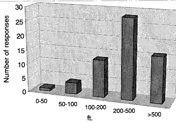
Figure 21. Operating/stand-off distance.
