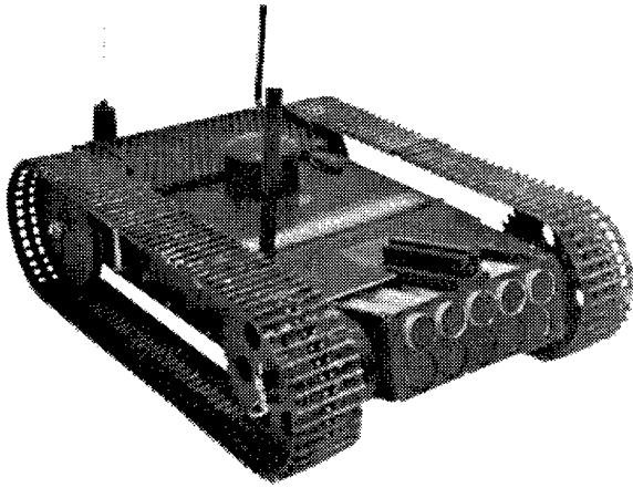
Figure 41. Lemming robot with less-lethal weapon launcher (left) and breaching saw (right).
