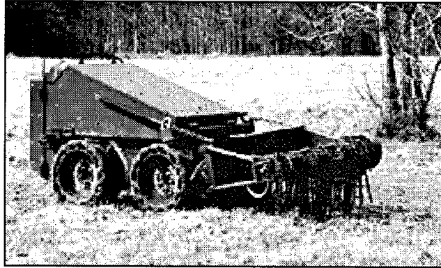
Figure 40. Mini-Flail.
