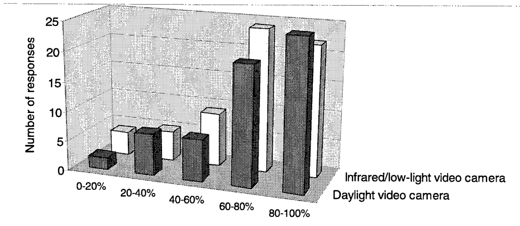
Figure 15. Video cameras.
