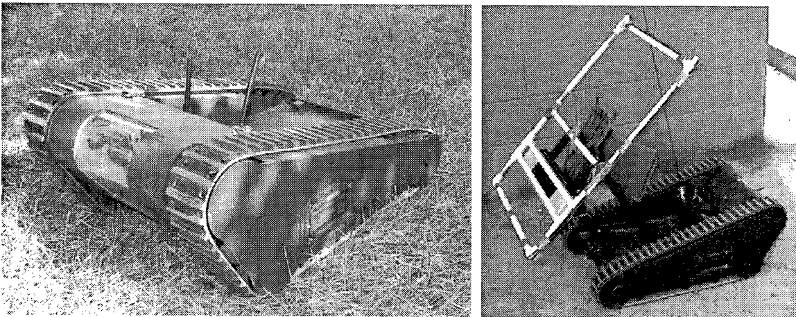
Figure 38. MATILDA robot (left) and MATILDA with breaching mechanism (right).
