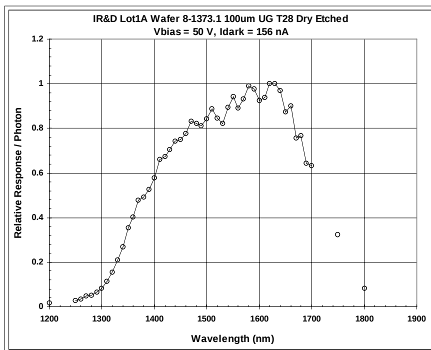
Figure 4. Spectral Characteristics of LPE HgCdTe APDs Fabricated for the CELRAP Program The diode design has been optimized to peak at 1.6 microns. QE is approximately 80% with no ARC.
