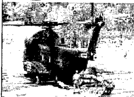
CH-53 — Range: 185 km radius Lift: 30,000 lbs (2 Wiesels) Wiesel — Crew: 2 Wt: 7900 lbs Armament: TOW/MK-20/Mortar/ADA
