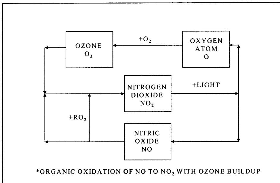
Figure I-2 Accumulation of ozone
