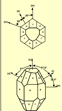
Common Crystallographic Planes in Sapphire
